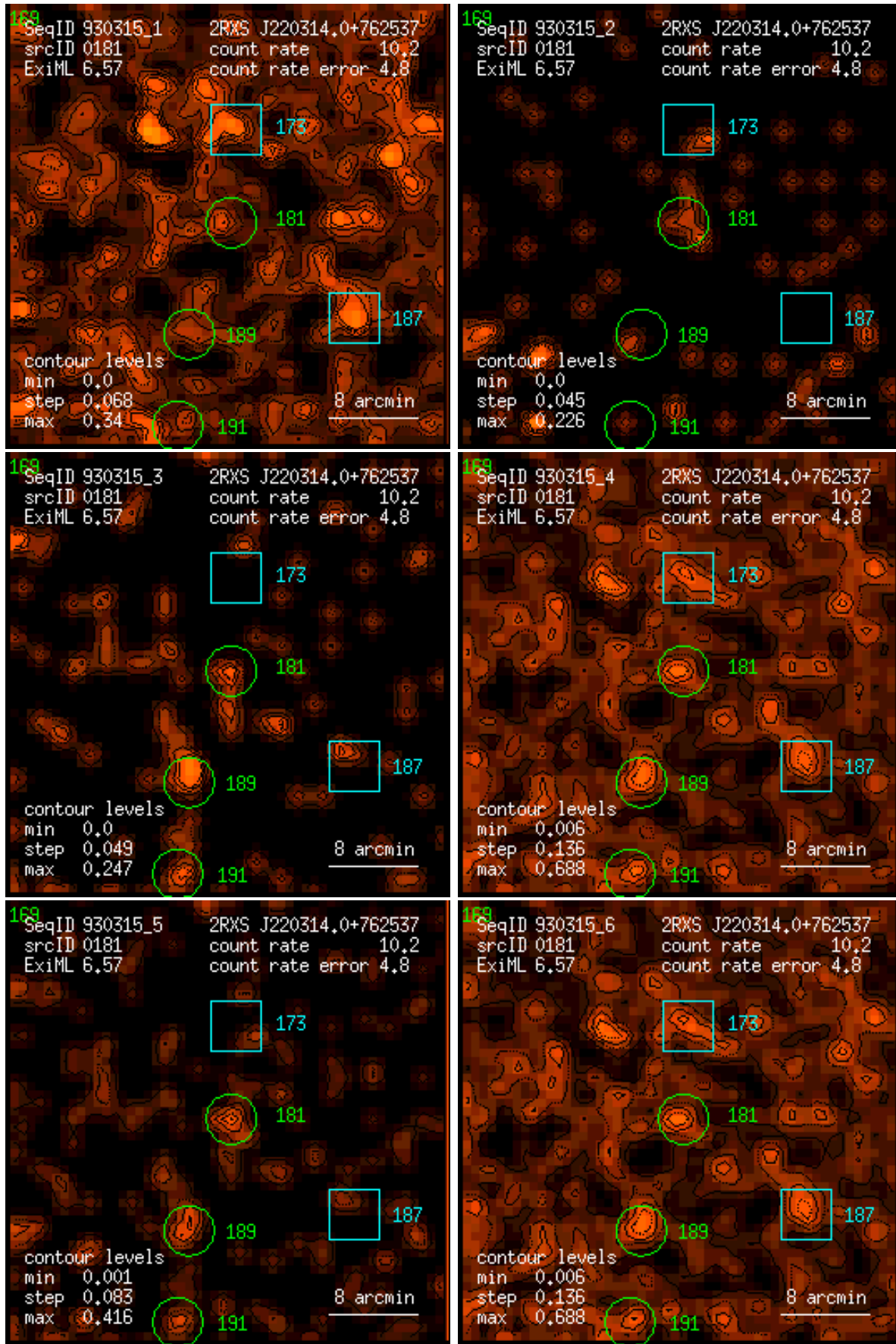
Figure 181: RASS 930315: detection 0181: band rate images, Gaussian filter: (1) PSPC channels 11 – 41, (2) 52 – 90, (3) 91 – 201, (4) 11 – 235, (5) 52 – 201, (6) 11 – 201. Broad band rates in counts/ks. Band rate contour levels in counts/ks/arcmin 2 .
