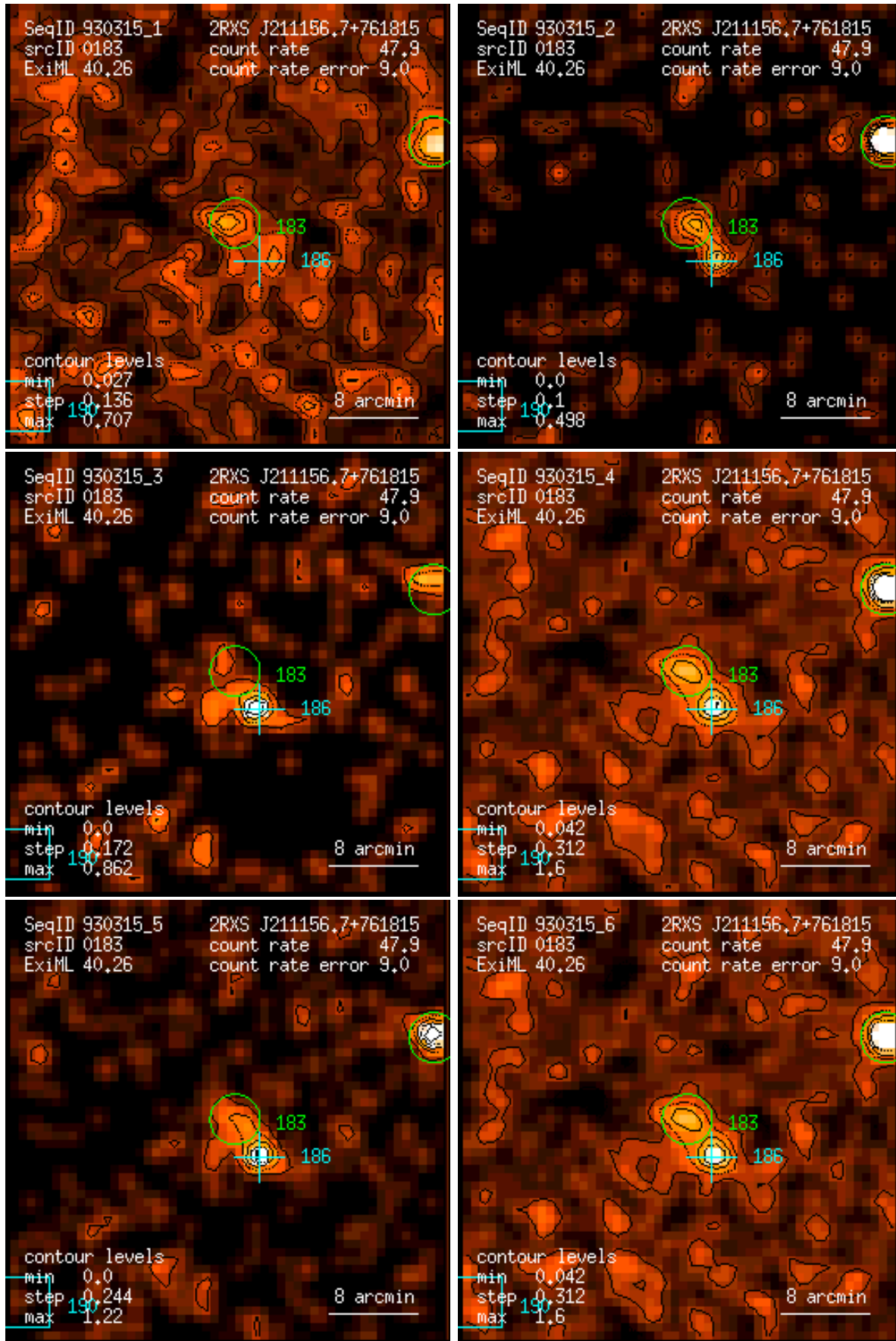
Figure 183: RASS 930315: detection 0183: band rate images, Gaussian filter: (1) PSPC channels 11 – 41, (2) 52 – 90, (3) 91 – 201, (4) 11 – 235, (5) 52 – 201, (6) 11 – 201. Broad band rates in counts/ks. Band rate contour levels in counts/ks/arcmin 2 .
