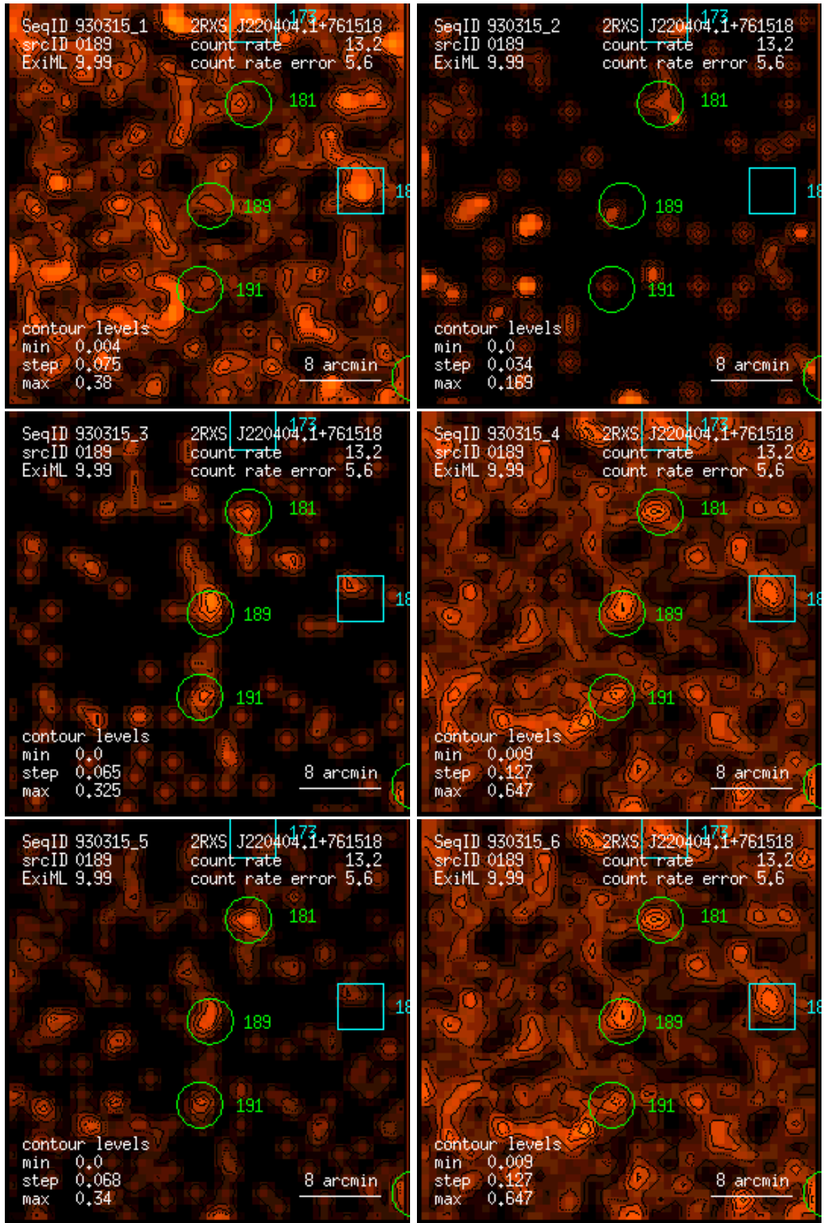
Figure 189: RASS 930315: detection 0189: band rate images, Gaussian filter: (1) PSPC channels 11 – 41, (2) 52 – 90, (3) 91 – 201, (4) 11 – 235, (5) 52 – 201, (6) 11 – 201. Broad band rates in counts/ks. Band rate contour levels in counts/ks/arcmin 2 .
