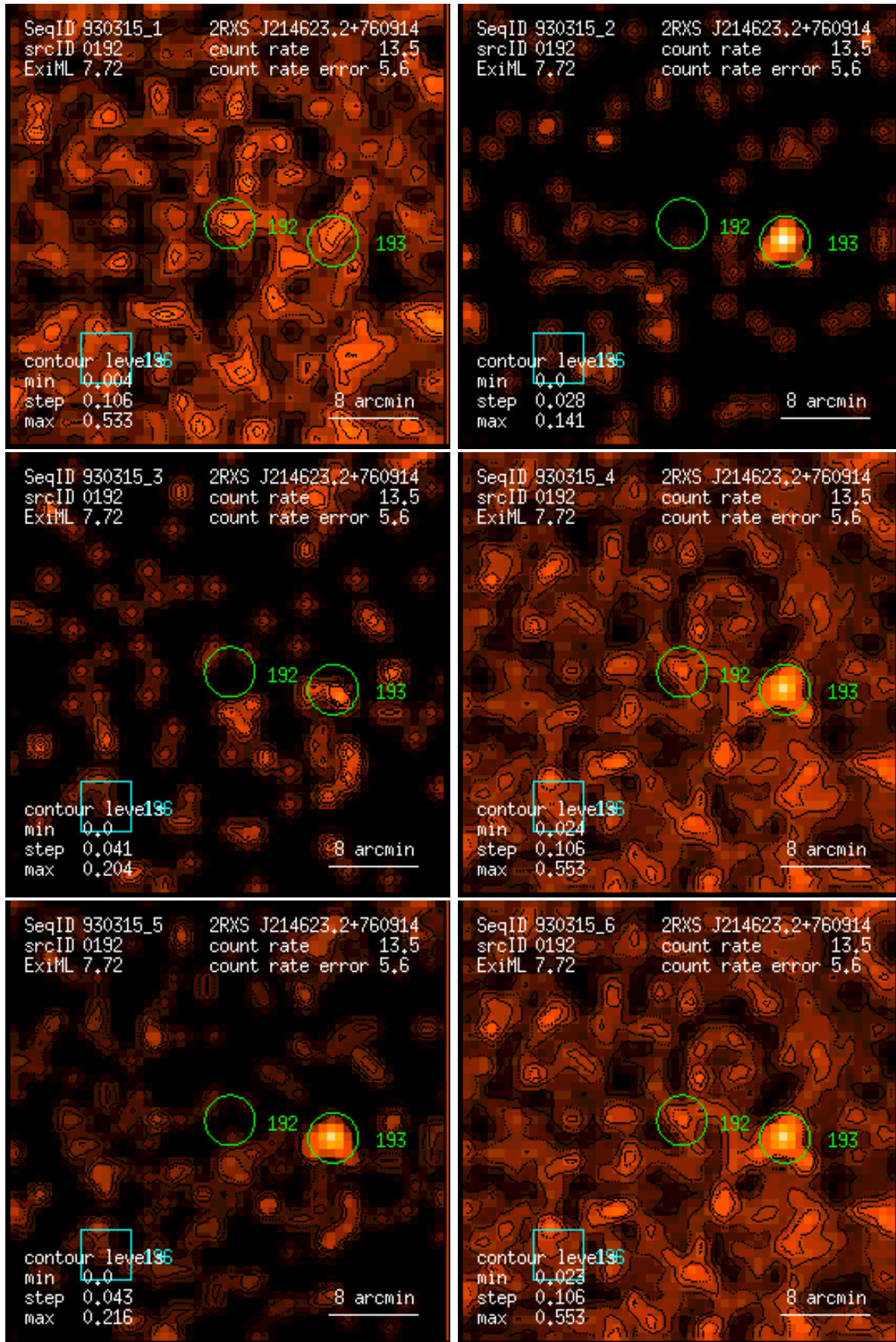
Figure 192: RASS 930315: detection 0192: band rate images, Gaussian filter: (1) PSPC channels 11 – 41, (2) 52 – 90, (3) 91 – 201, (4) 11 – 235, (5) 52 – 201, (6) 11 – 201. Broad band rates in counts/ks. Band rate contour levels in counts/ks/arcmin 2 .
