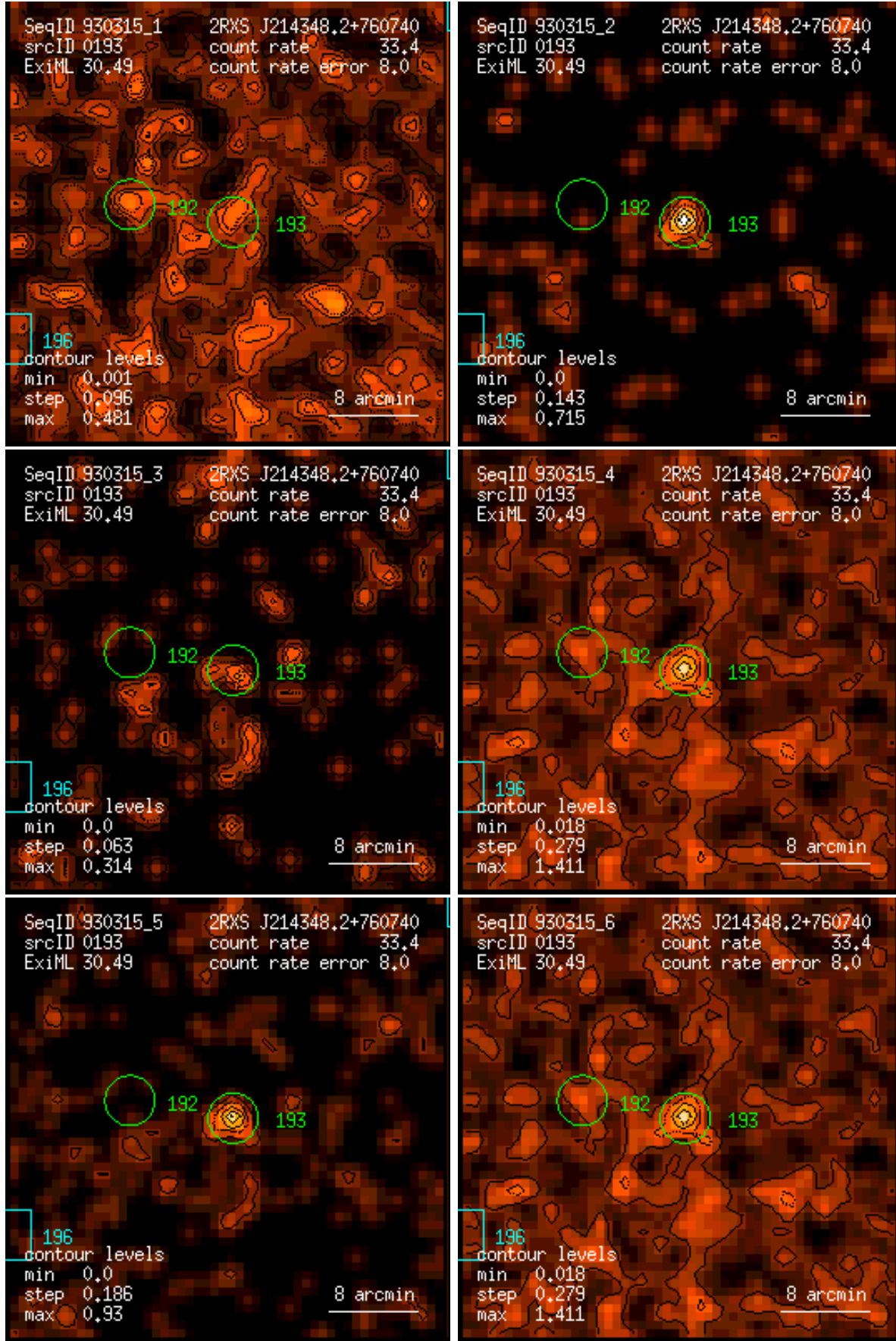
Figure 193: RASS 930315: detection 0193: band rate images, Gaussian filter: (1) PSPC channels 11 – 41, (2) 52 – 90, (3) 91 – 201, (4) 11 – 235, (5) 52 – 201, (6) 11 – 201. Broad band rates in counts/ks. Band rate contour levels in counts/ks/arcmin 2 .
