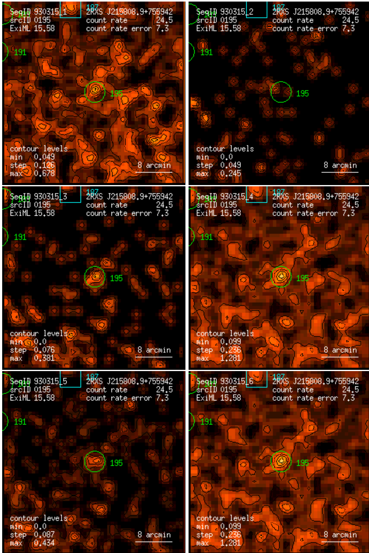
Figure 195: RASS 930315: detection 0195: band rate images, Gaussian filter: (1) PSPC channels 11 – 41, (2) 52 – 90, (3) 91 – 201, (4) 11 – 235, (5) 52 – 201, (6) 11 – 201. Broad band rates in counts/ks. Band rate contour levels in counts/ks/arcmin 2 .
