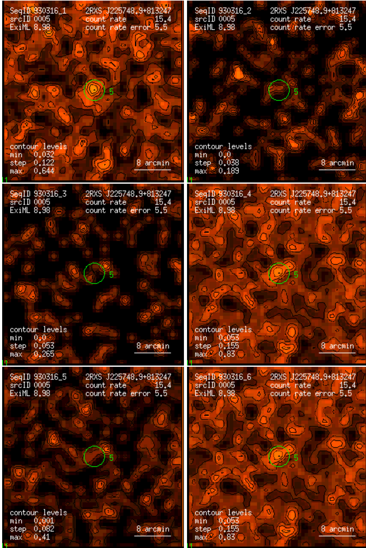
Figure 5: RASS 930316: detection 0005: band rate images, Gaussian filter: (1) PSPC channels 11 – 41, (2) 52 – 90, (3) 91 – 201, (4) 11 – 235, (5) 52 – 201, (6) 11 – 201. Broad band rates in counts/ks. Band rate contour levels in counts/ks/arcmin 2 .
