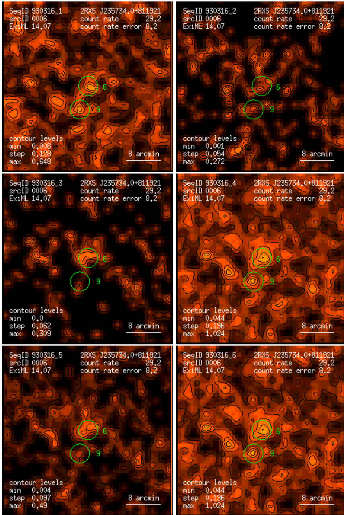
Figure 6: RASS 930316: detection 0006: band rate images, Gaussian filter: (1) PSPC channels 11 – 41, (2) 52 – 90, (3) 91 – 201, (4) 11 – 235, (5) 52 – 201, (6) 11 – 201. Broad band rates in counts/ks. Band rate contour levels in counts/ks/arcmin 2 .
