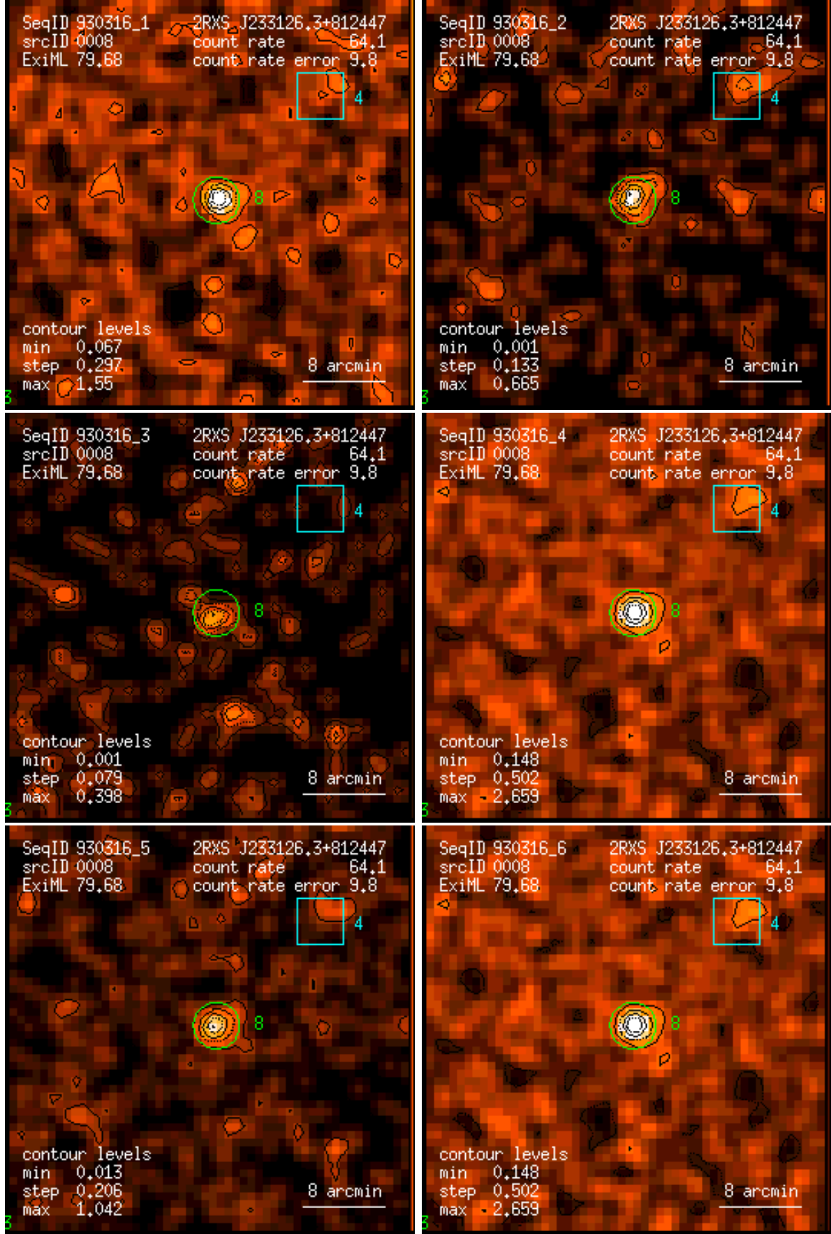
Figure 8: RASS 930316: detection 0008: band rate images, Gaussian filter: (1) PSPC channels 11 – 41, (2) 52 – 90, (3) 91 – 201, (4) 11 – 235, (5) 52 – 201, (6) 11 – 201. Broad band rates in counts/ks. Band rate contour levels in counts/ks/arcmin 2 .
