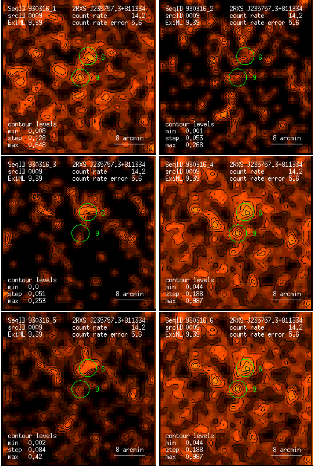
Figure 9: RASS 930316: detection 0009: band rate images, Gaussian filter: (1) PSPC channels 11 – 41, (2) 52 – 90, (3) 91 – 201, (4) 11 – 235, (5) 52 – 201, (6) 11 – 201. Broad band rates in counts/ks. Band rate contour levels in counts/ks/arcmin 2 .
