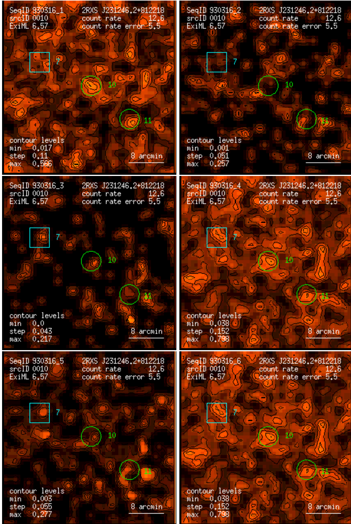
Figure 10: RASS 930316: detection 0010: band rate images, Gaussian filter: (1) PSPC channels 11 – 41, (2) 52 – 90, (3) 91 – 201, (4) 11 – 235, (5) 52 – 201, (6) 11 – 201. Broad band rates in counts/ks. Band rate contour levels in counts/ks/arcmin 2 .
