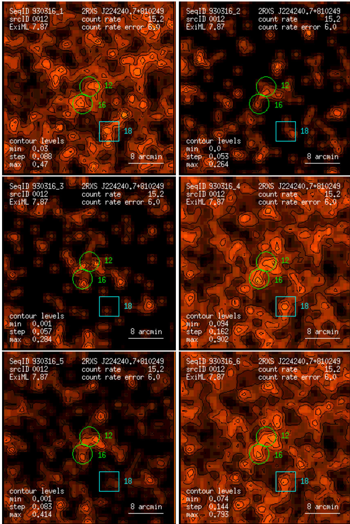
Figure 12: RASS 930316: detection 0012: band rate images, Gaussian filter: (1) PSPC channels 11 – 41, (2) 52 – 90, (3) 91 – 201, (4) 11 – 235, (5) 52 – 201, (6) 11 – 201. Broad band rates in counts/ks. Band rate contour levels in counts/ks/arcmin 2 .
