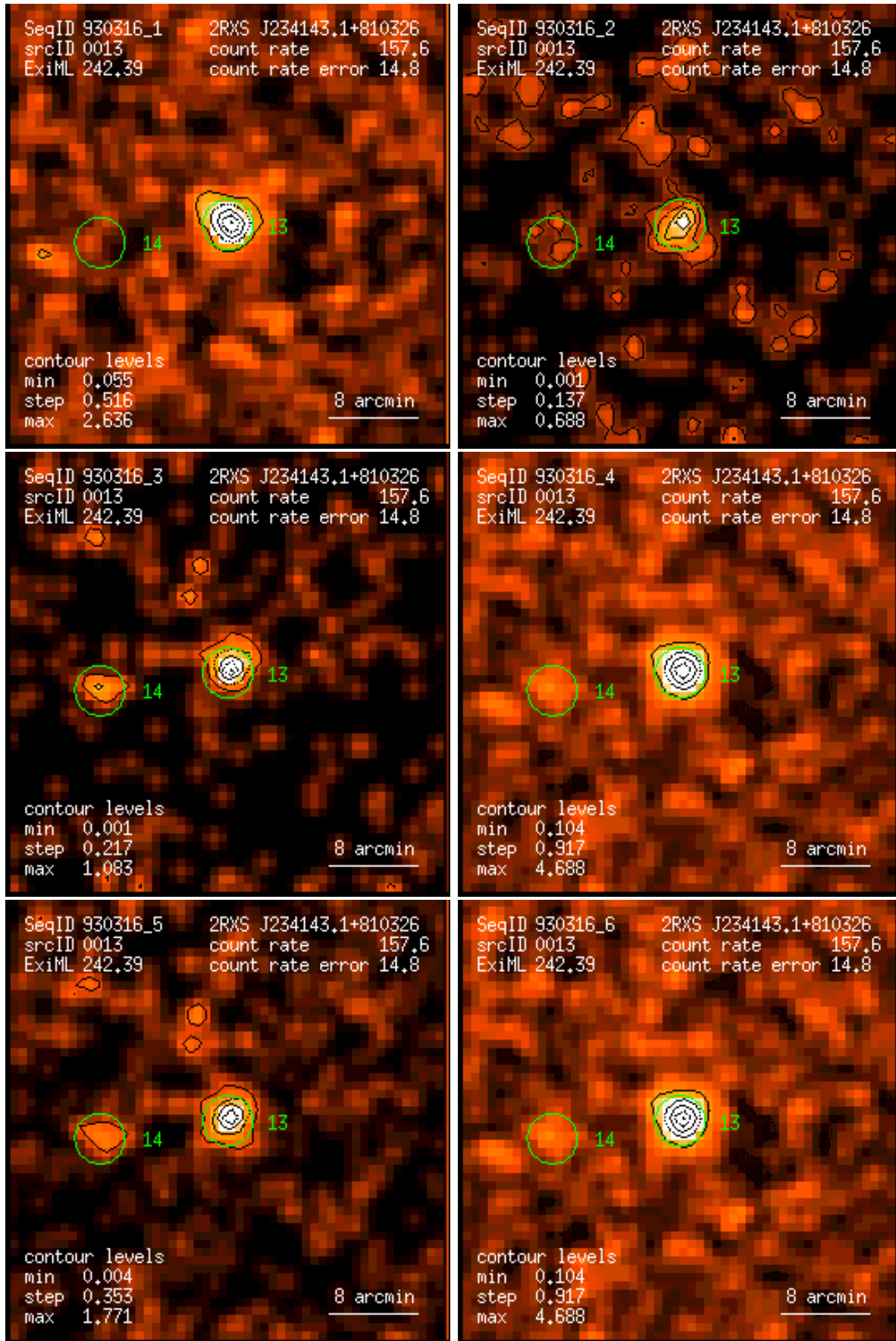
Figure 13: RASS 930316: detection 0013: band rate images, Gaussian filter: (1) PSPC channels 11 – 41, (2) 52 – 90, (3) 91 – 201, (4) 11 – 235, (5) 52 – 201, (6) 11 – 201. Broad band rates in counts/ks. Band rate contour levels in counts/ks/arcmin 2 .
