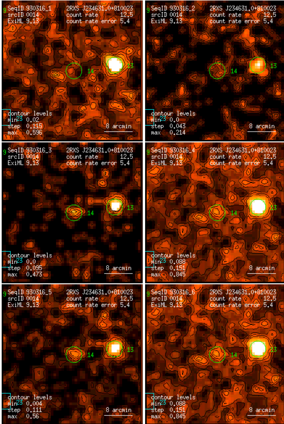
Figure 14: RASS 930316: detection 0014: band rate images, Gaussian filter: (1) PSPC channels 11 – 41, (2) 52 – 90, (3) 91 – 201, (4) 11 – 235, (5) 52 – 201, (6) 11 – 201. Broad band rates in counts/ks. Band rate contour levels in counts/ks/arcmin 2 .
