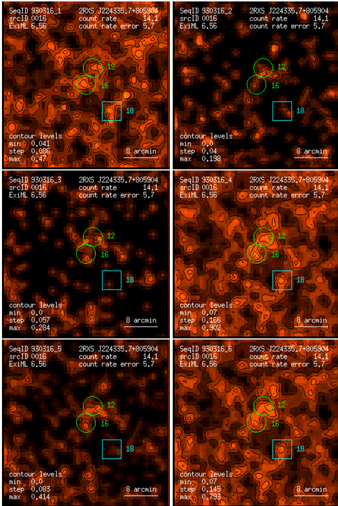
Figure 16: RASS 930316: detection 0016: band rate images, Gaussian filter: (1) PSPC channels 11 – 41, (2) 52 – 90, (3) 91 – 201, (4) 11 – 235, (5) 52 – 201, (6) 11 – 201. Broad band rates in counts/ks. Band rate contour levels in counts/ks/arcmin 2 .
