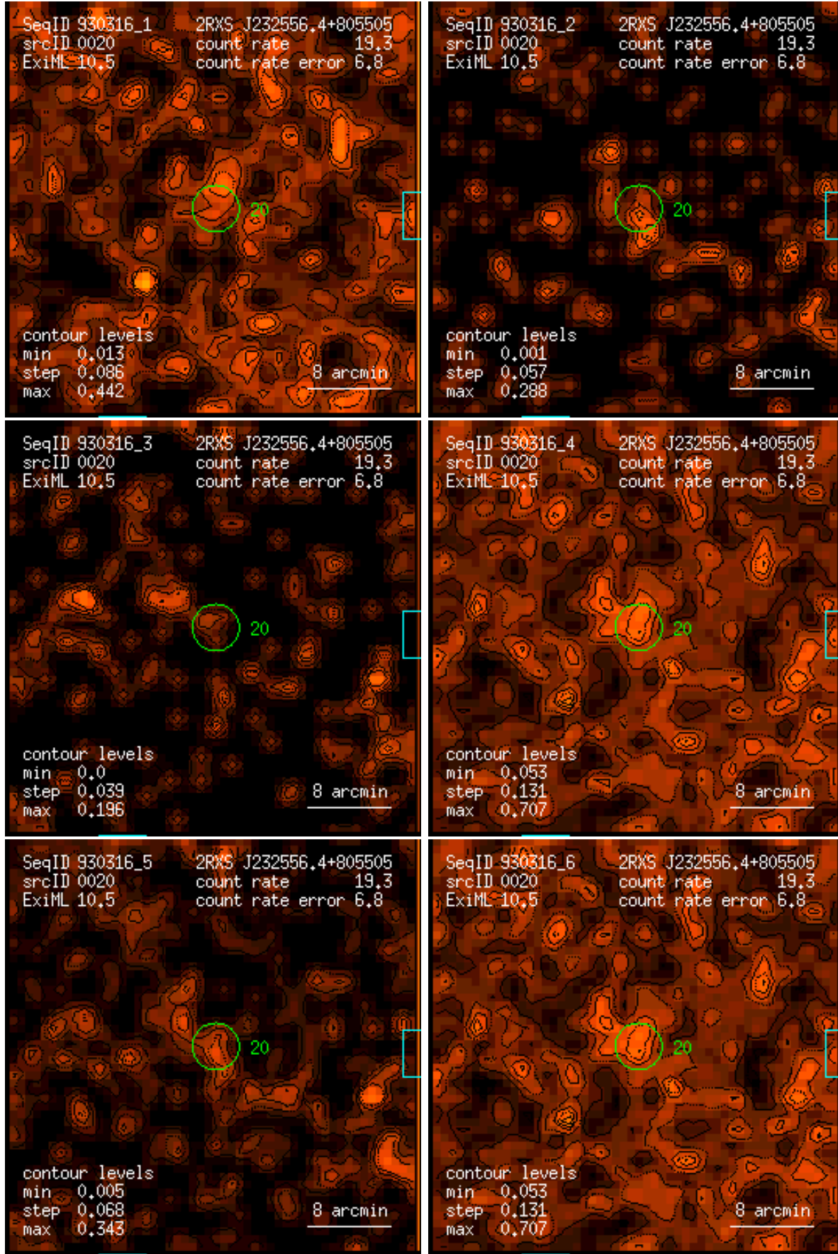
Figure 20: RASS 930316: detection 0020: band rate images, Gaussian filter: (1) PSPC channels 11 – 41, (2) 52 – 90, (3) 91 – 201, (4) 11 – 235, (5) 52 – 201, (6) 11 – 201. Broad band rates in counts/ks. Band rate contour levels in counts/ks/arcmin 2 .
