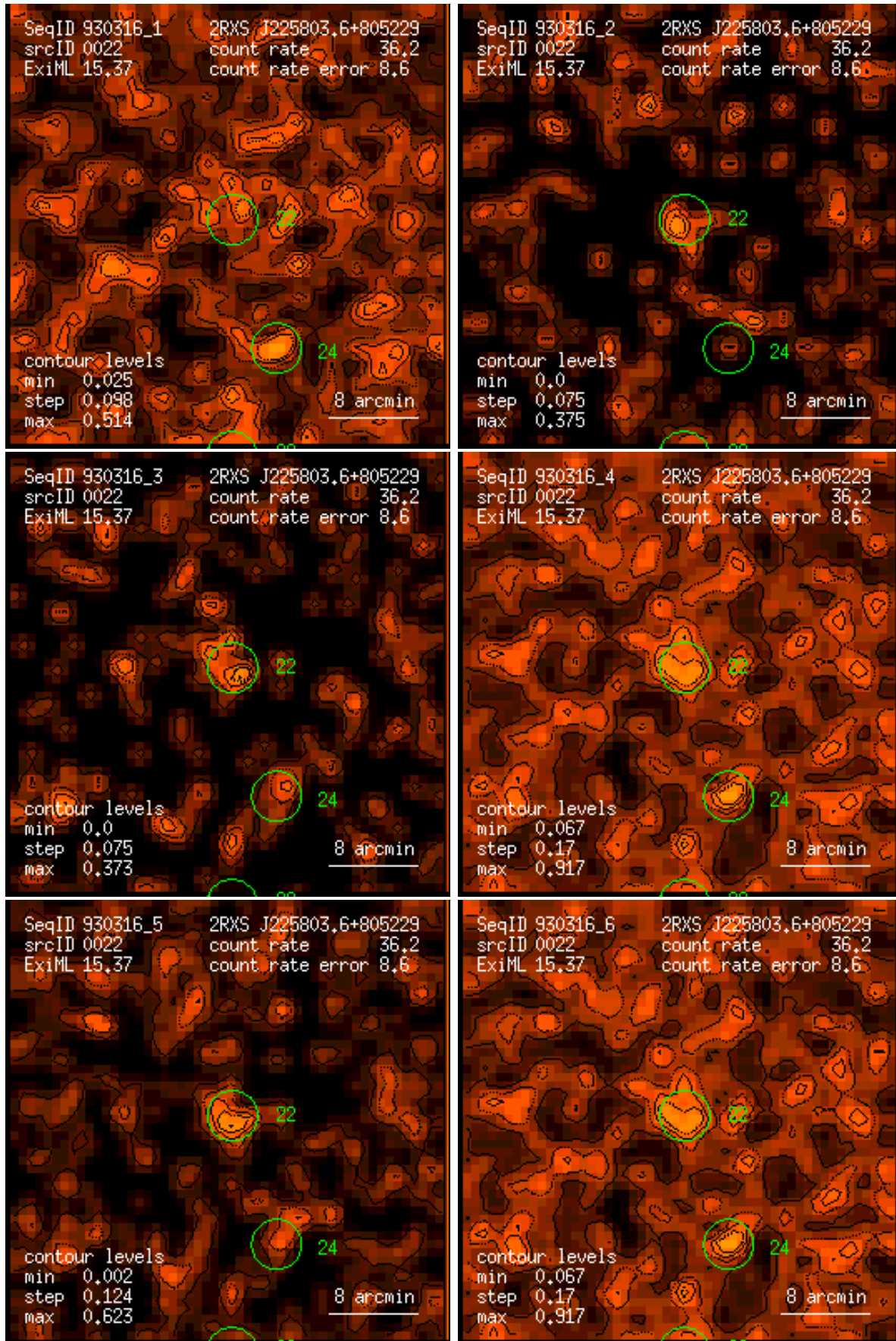
Figure 22: RASS 930316: detection 0022: band rate images, Gaussian filter: (1) PSPC channels 11 – 41, (2) 52 – 90, (3) 91 – 201, (4) 11 – 235, (5) 52 – 201, (6) 11 – 201. Broad band rates in counts/ks. Band rate contour levels in counts/ks/arcmin 2 .
