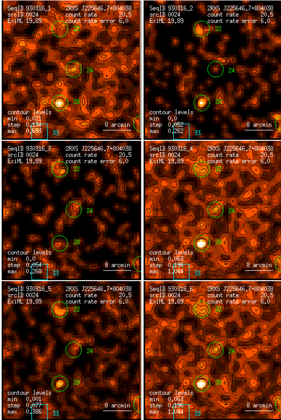
Figure 24: RASS 930316: detection 0024: band rate images, Gaussian filter: (1) PSPC channels 11 – 41, (2) 52 – 90, (3) 91 – 201, (4) 11 – 235, (5) 52 – 201, (6) 11 – 201. Broad band rates in counts/ks. Band rate contour levels in counts/ks/arcmin 2 .
