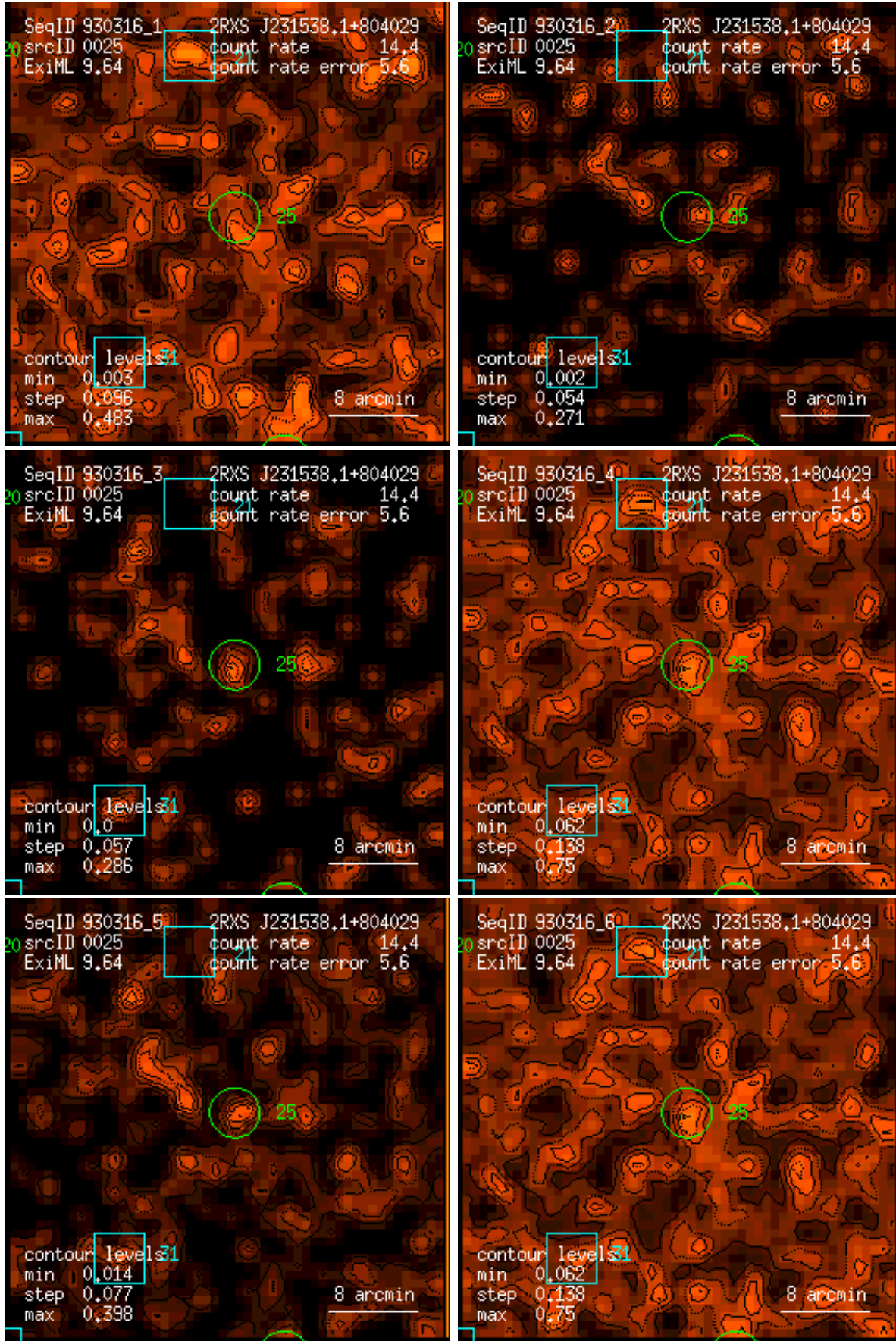
Figure 25: RASS 930316: detection 0025: band rate images, Gaussian filter: (1) PSPC channels 11 – 41, (2) 52 – 90, (3) 91 – 201, (4) 11 – 235, (5) 52 – 201, (6) 11 – 201. Broad band rates in counts/ks. Band rate contour levels in counts/ks/arcmin 2 .
