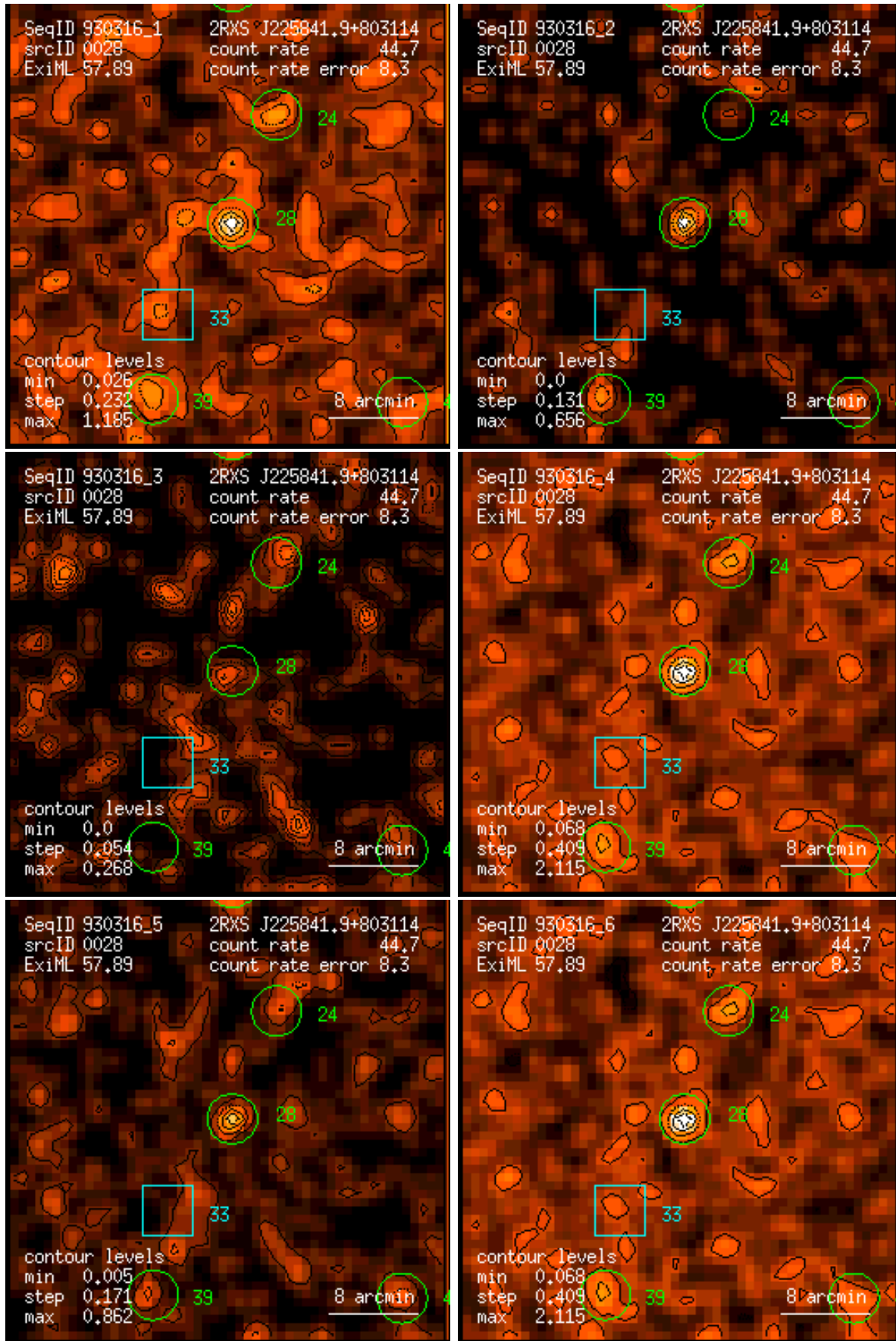
Figure 28: RASS 930316: detection 0028: band rate images, Gaussian filter: (1) PSPC channels 11 – 41, (2) 52 – 90, (3) 91 – 201, (4) 11 – 235, (5) 52 – 201, (6) 11 – 201. Broad band rates in counts/ks. Band rate contour levels in counts/ks/arcmin 2 .
