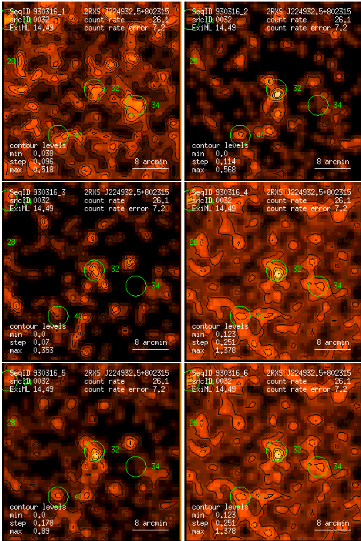
Figure 32: RASS 930316: detection 0032: band rate images, Gaussian filter: (1) PSPC channels 11 – 41, (2) 52 – 90, (3) 91 – 201, (4) 11 – 235, (5) 52 – 201, (6) 11 – 201. Broad band rates in counts/ks. Band rate contour levels in counts/ks/arcmin 2 .
