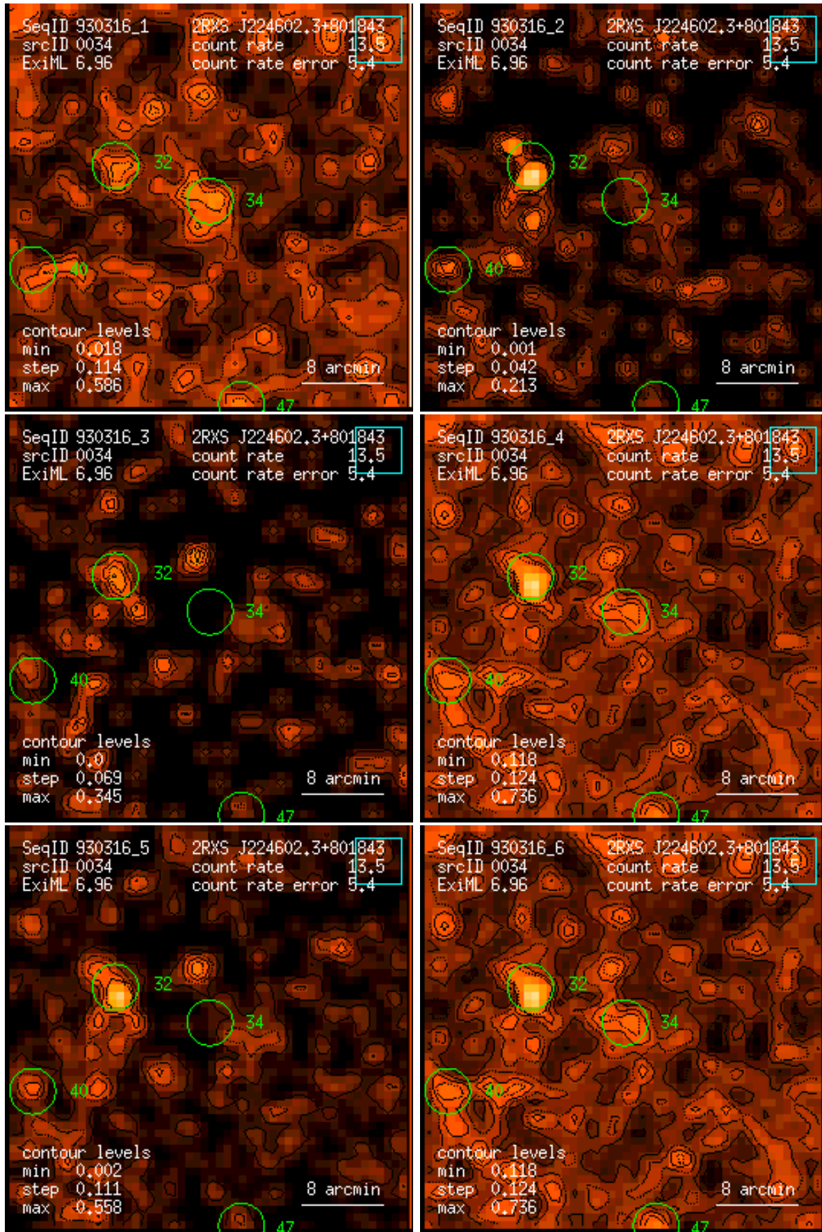
Figure 34: RASS 930316: detection 0034: band rate images, Gaussian filter: (1) PSPC channels 11 – 41, (2) 52 – 90, (3) 91 – 201, (4) 11 – 235, (5) 52 – 201, (6) 11 – 201. Broad band rates in counts/ks. Band rate contour levels in counts/ks/arcmin 2 .
