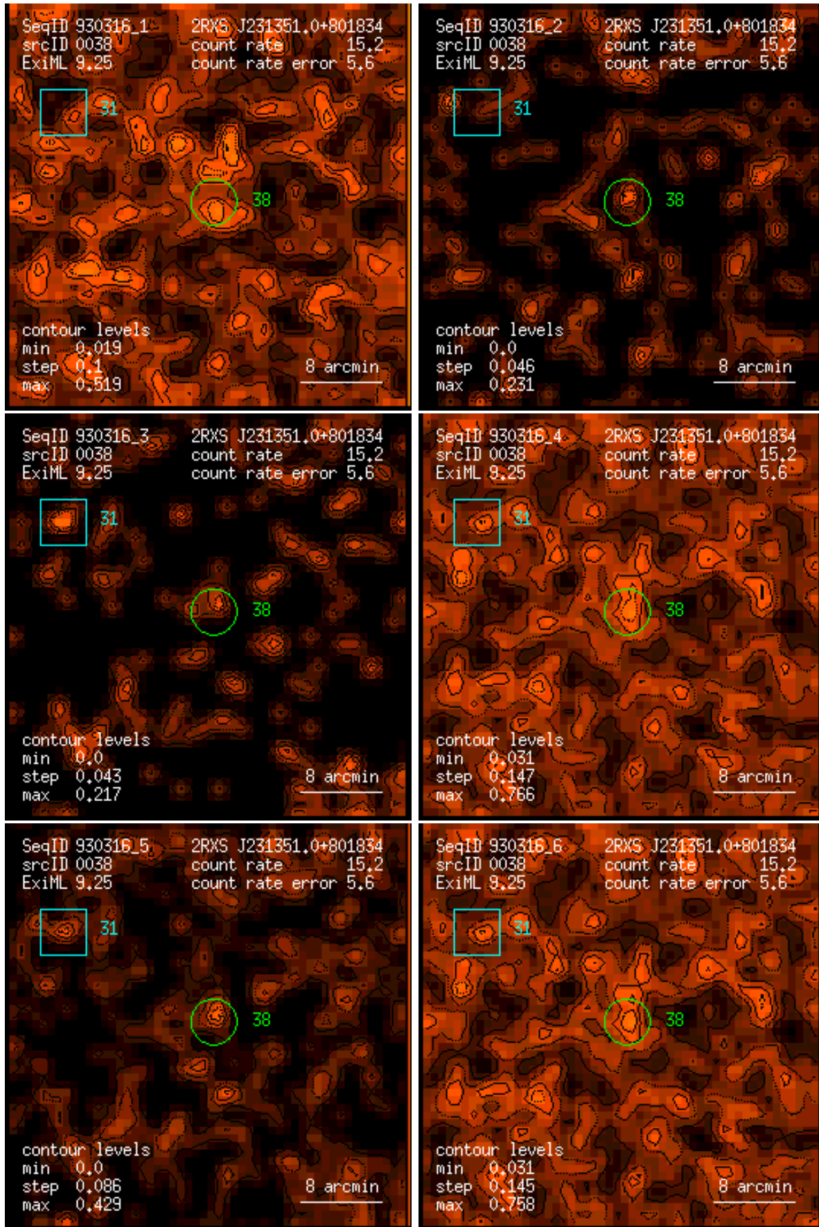
Figure 38: RASS 930316: detection 0038: band rate images, Gaussian filter: (1) PSPC channels 11 – 41, (2) 52 – 90, (3) 91 – 201, (4) 11 – 235, (5) 52 – 201, (6) 11 – 201. Broad band rates in counts/ks. Band rate contour levels in counts/ks/arcmin 2 .
