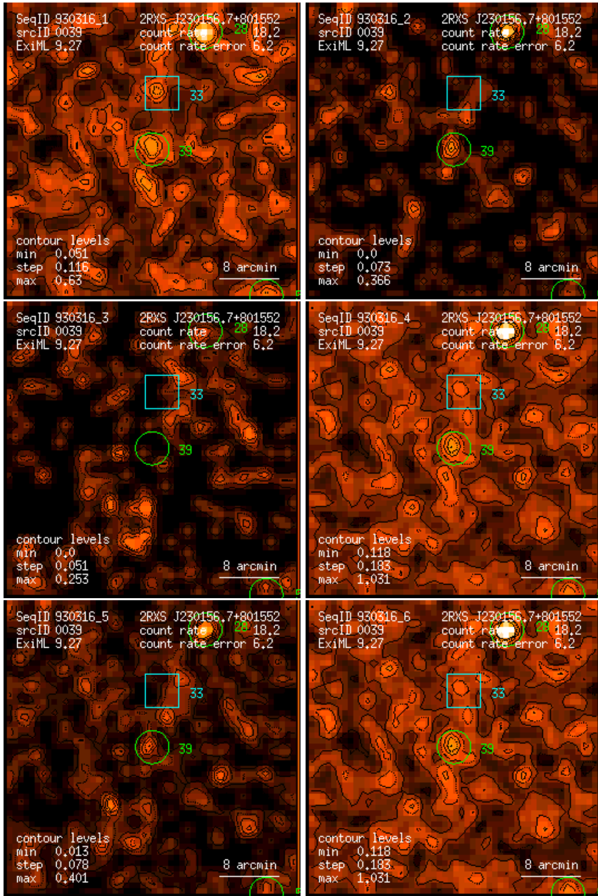
Figure 39: RASS 930316: detection 0039: band rate images, Gaussian filter: (1) PSPC channels 11 – 41, (2) 52 – 90, (3) 91 – 201, (4) 11 – 235, (5) 52 – 201, (6) 11 – 201. Broad band rates in counts/ks. Band rate contour levels in counts/ks/arcmin 2 .
