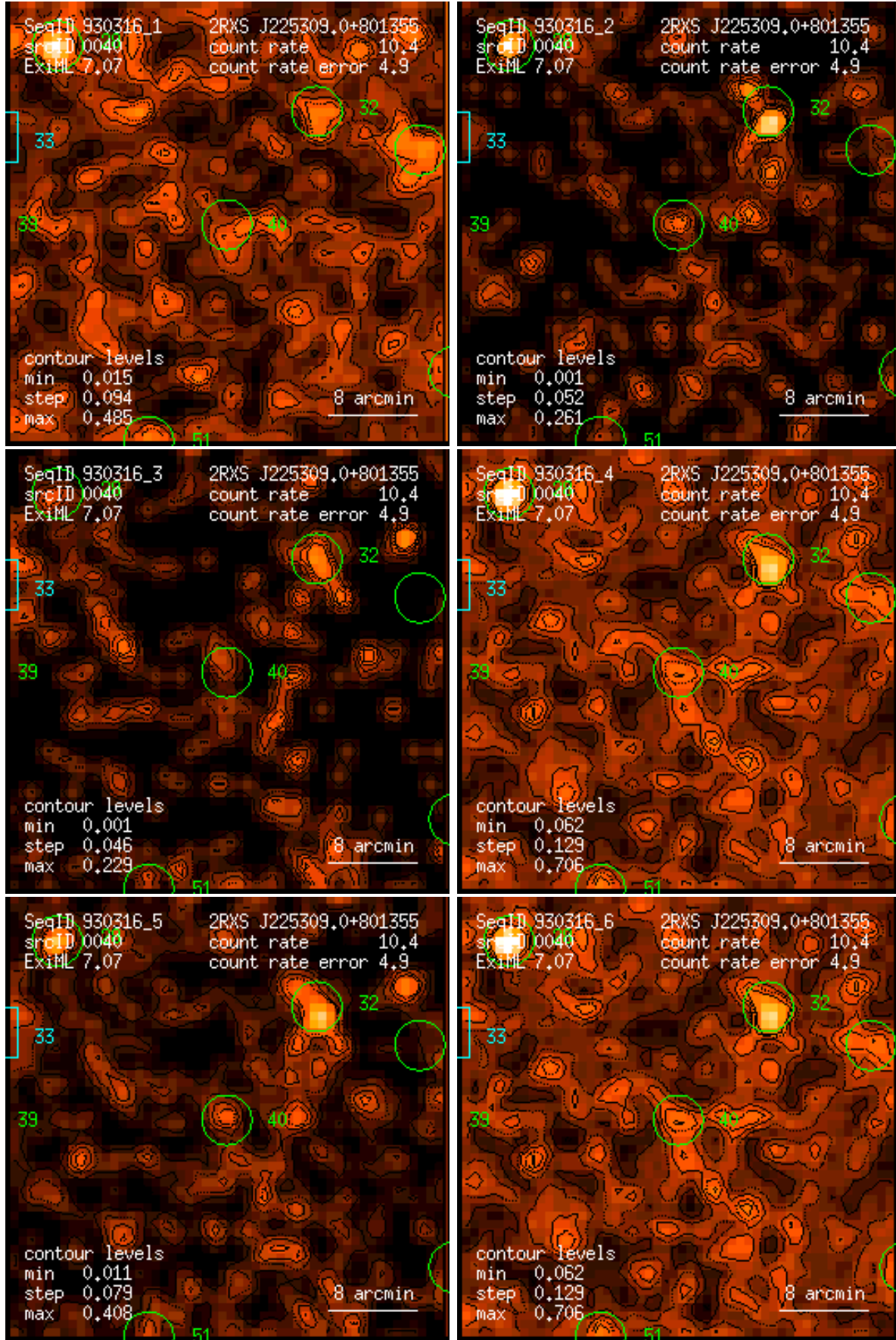
Figure 40: RASS 930316: detection 0040: band rate images, Gaussian filter: (1) PSPC channels 11 – 41, (2) 52 – 90, (3) 91 – 201, (4) 11 – 235, (5) 52 – 201, (6) 11 – 201. Broad band rates in counts/ks. Band rate contour levels in counts/ks/arcmin 2 .
