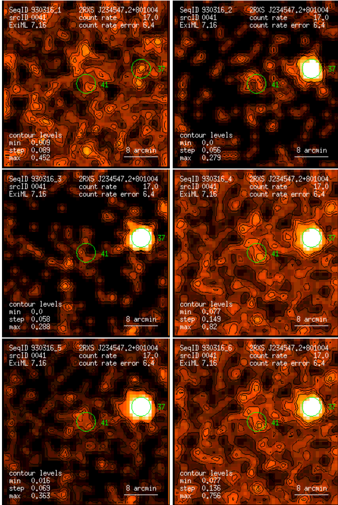
Figure 41: RASS 930316: detection 0041: band rate images, Gaussian filter: (1) PSPC channels 11 – 41, (2) 52 – 90, (3) 91 – 201, (4) 11 – 235, (5) 52 – 201, (6) 11 – 201. Broad band rates in counts/ks. Band rate contour levels in counts/ks/arcmin 2 .
