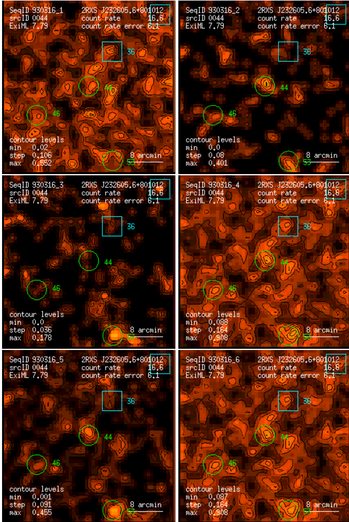
Figure 44: RASS 930316: detection 0044: band rate images, Gaussian filter: (1) PSPC channels 11 – 41, (2) 52 – 90, (3) 91 – 201, (4) 11 – 235, (5) 52 – 201, (6) 11 – 201. Broad band rates in counts/ks. Band rate contour levels in counts/ks/arcmin 2 .
