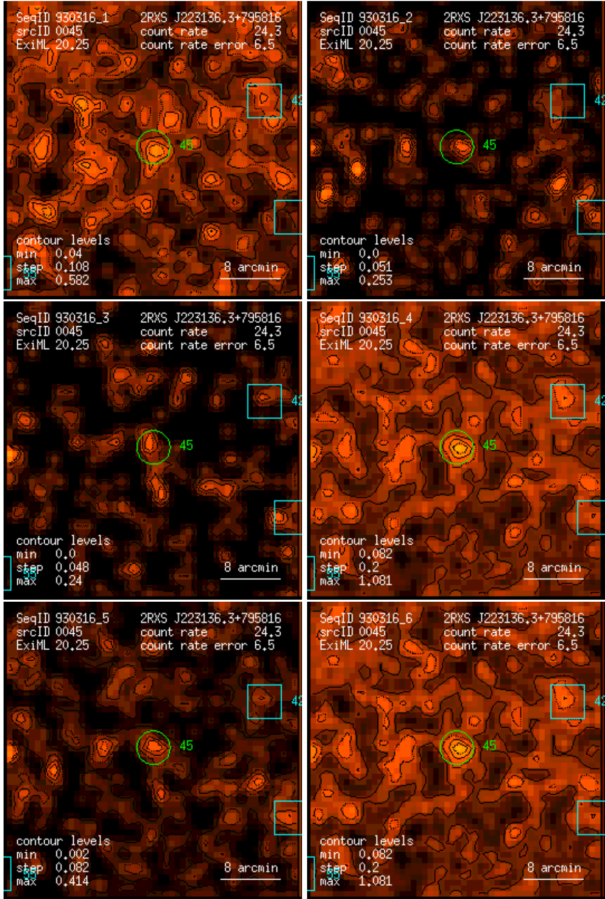
Figure 45: RASS 930316: detection 0045: band rate images, Gaussian filter: (1) PSPC channels 11 – 41, (2) 52 – 90, (3) 91 – 201, (4) 11 – 235, (5) 52 – 201, (6) 11 – 201. Broad band rates in counts/ks. Band rate contour levels in counts/ks/arcmin 2 .
