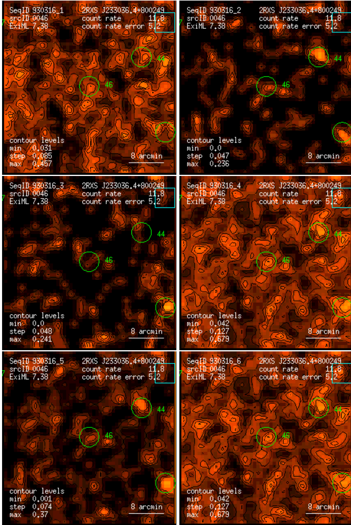
Figure 46: RASS 930316: detection 0046: band rate images, Gaussian filter: (1) PSPC channels 11 – 41, (2) 52 – 90, (3) 91 – 201, (4) 11 – 235, (5) 52 – 201, (6) 11 – 201. Broad band rates in counts/ks. Band rate contour levels in counts/ks/arcmin 2 .
