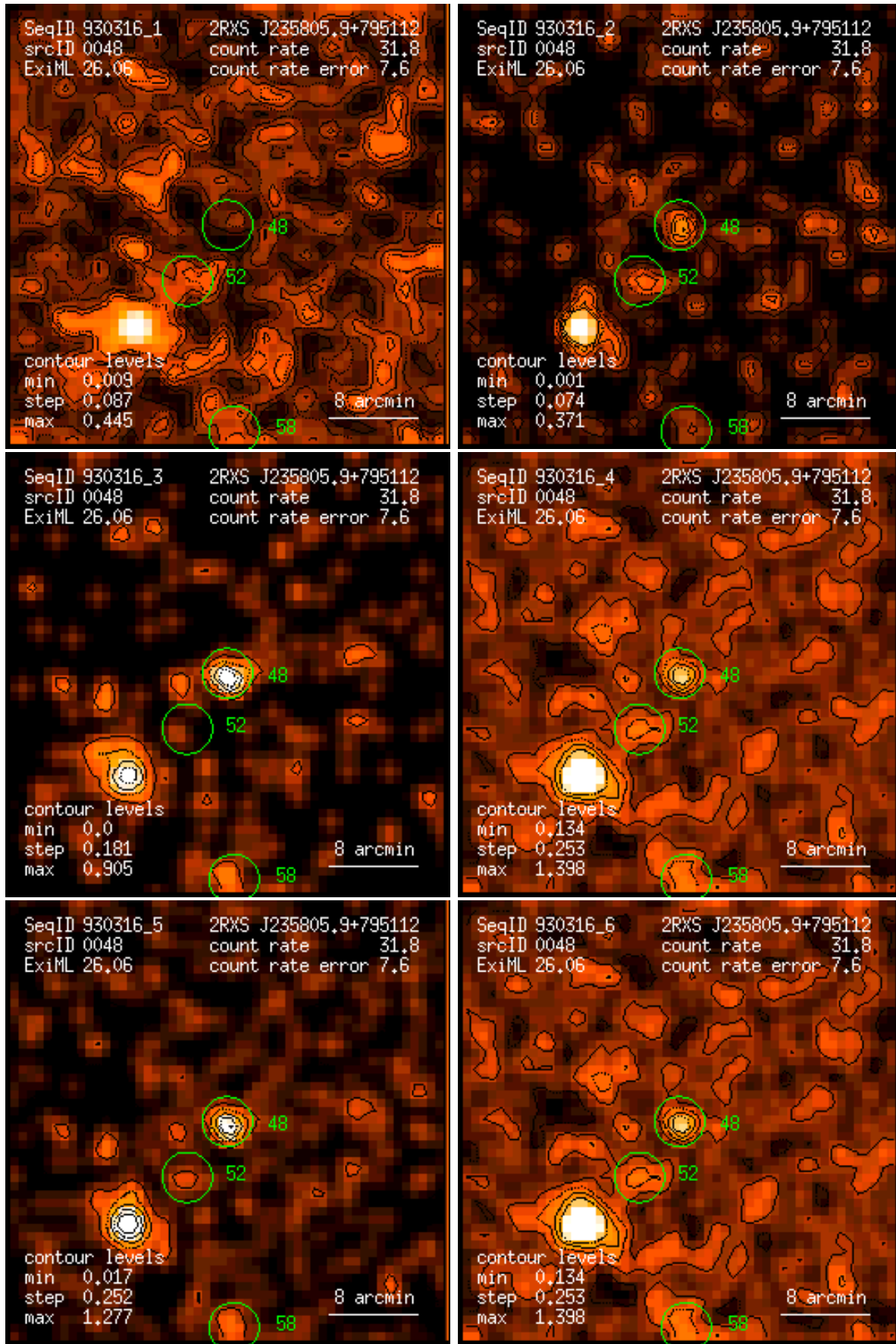
Figure 48: RASS 930316: detection 0048: band rate images, Gaussian filter: (1) PSPC channels 11 – 41, (2) 52 – 90, (3) 91 – 201, (4) 11 – 235, (5) 52 – 201, (6) 11 – 201. Broad band rates in counts/ks. Band rate contour levels in counts/ks/arcmin 2 .
