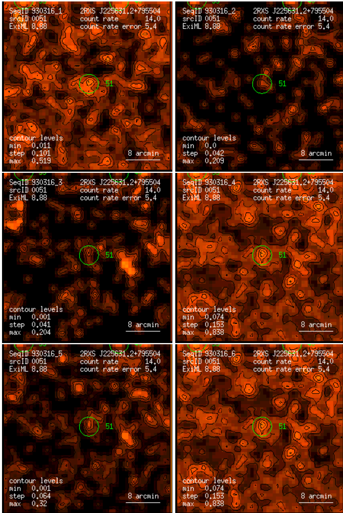
Figure 51: RASS 930316: detection 0051: band rate images, Gaussian filter: (1) PSPC channels 11 – 41, (2) 52 – 90, (3) 91 – 201, (4) 11 – 235, (5) 52 – 201, (6) 11 – 201. Broad band rates in counts/ks. Band rate contour levels in counts/ks/arcmin 2 .
