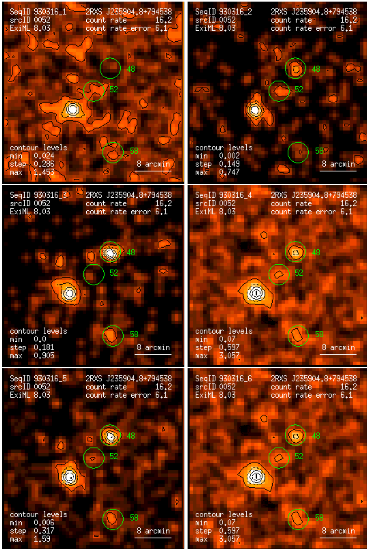
Figure 52: RASS 930316: detection 0052: band rate images, Gaussian filter: (1) PSPC channels 11 – 41, (2) 52 – 90, (3) 91 – 201, (4) 11 – 235, (5) 52 – 201, (6) 11 – 201. Broad band rates in counts/ks. Band rate contour levels in counts/ks/arcmin 2 .
