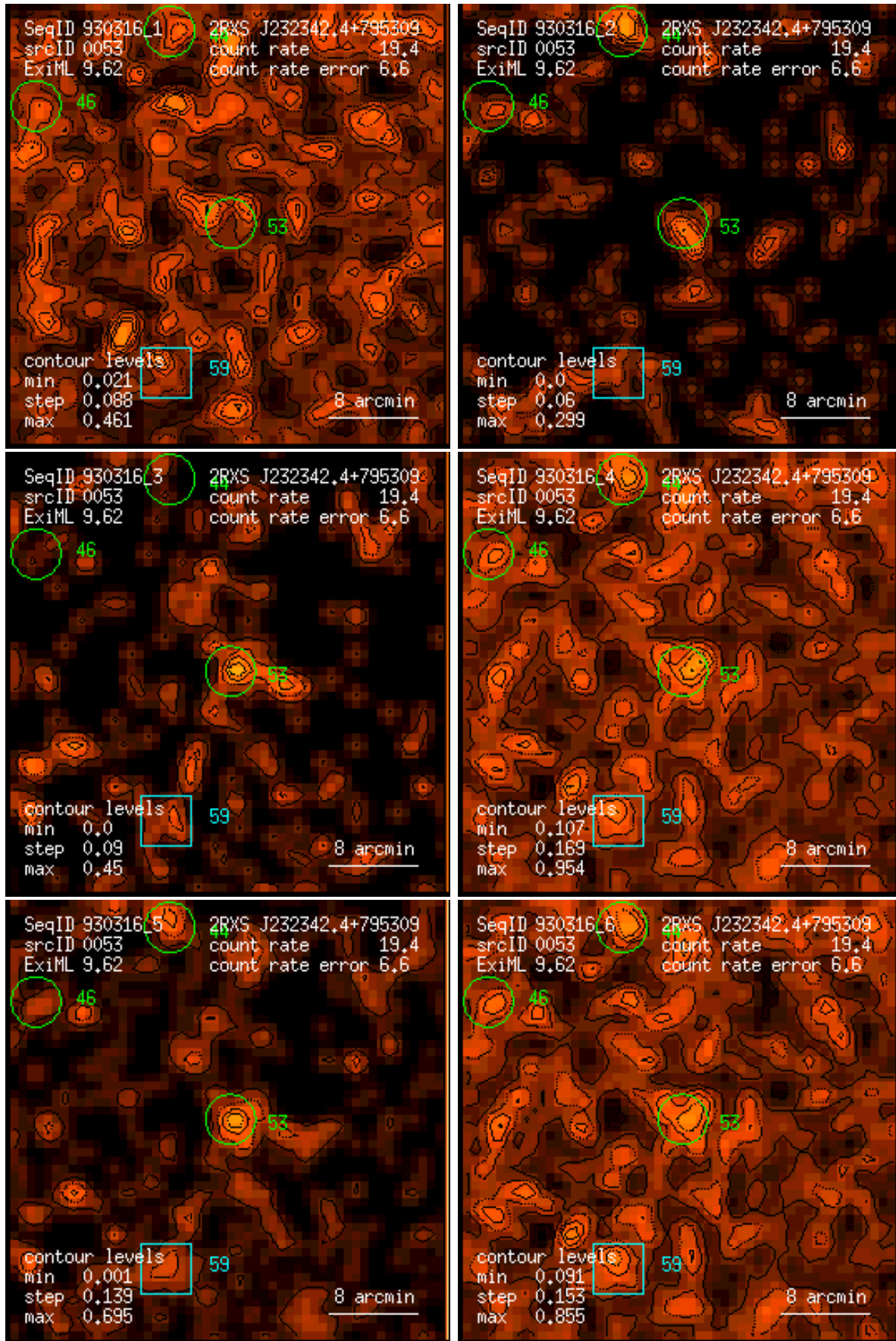
Figure 53: RASS 930316: detection 0053: band rate images, Gaussian filter: (1) PSPC channels 11 – 41, (2) 52 – 90, (3) 91 – 201, (4) 11 – 235, (5) 52 – 201, (6) 11 – 201. Broad band rates in counts/ks. Band rate contour levels in counts/ks/arcmin 2 .
