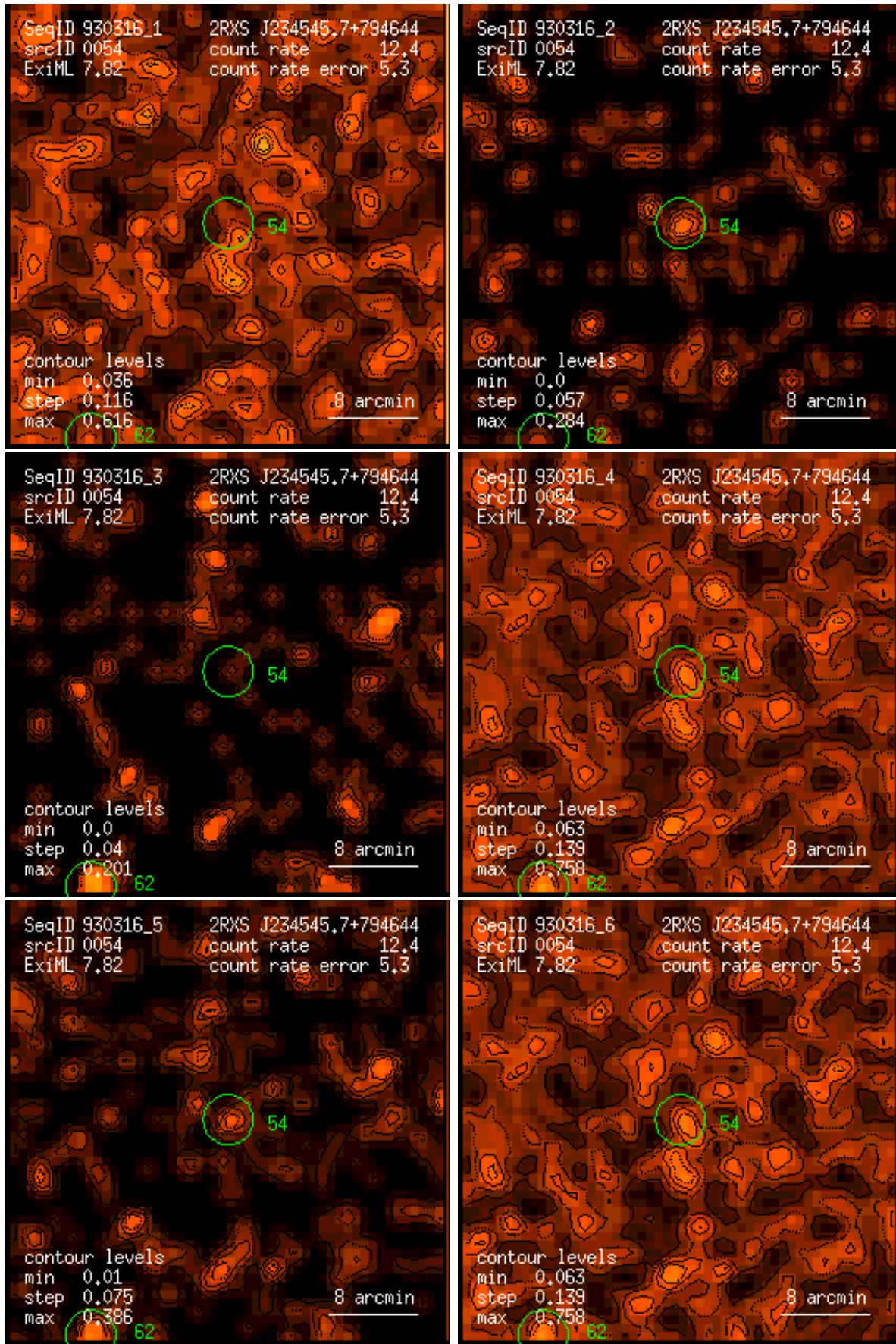
Figure 54: RASS 930316: detection 0054: band rate images, Gaussian filter: (1) PSPC channels 11 – 41, (2) 52 – 90, (3) 91 – 201, (4) 11 – 235, (5) 52 – 201, (6) 11 – 201. Broad band rates in counts/ks. Band rate contour levels in counts/ks/arcmin 2 .
