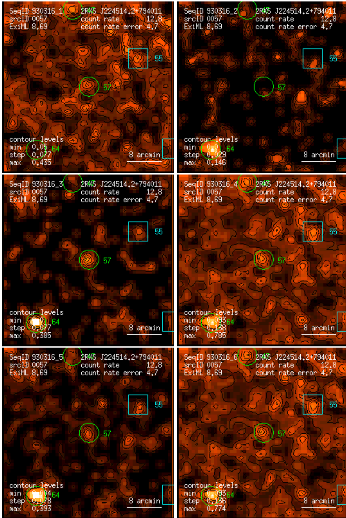
Figure 57: RASS 930316: detection 0057: band rate images, Gaussian filter: (1) PSPC channels 11 – 41, (2) 52 – 90, (3) 91 – 201, (4) 11 – 235, (5) 52 – 201, (6) 11 – 201. Broad band rates in counts/ks. Band rate contour levels in counts/ks/arcmin 2 .
