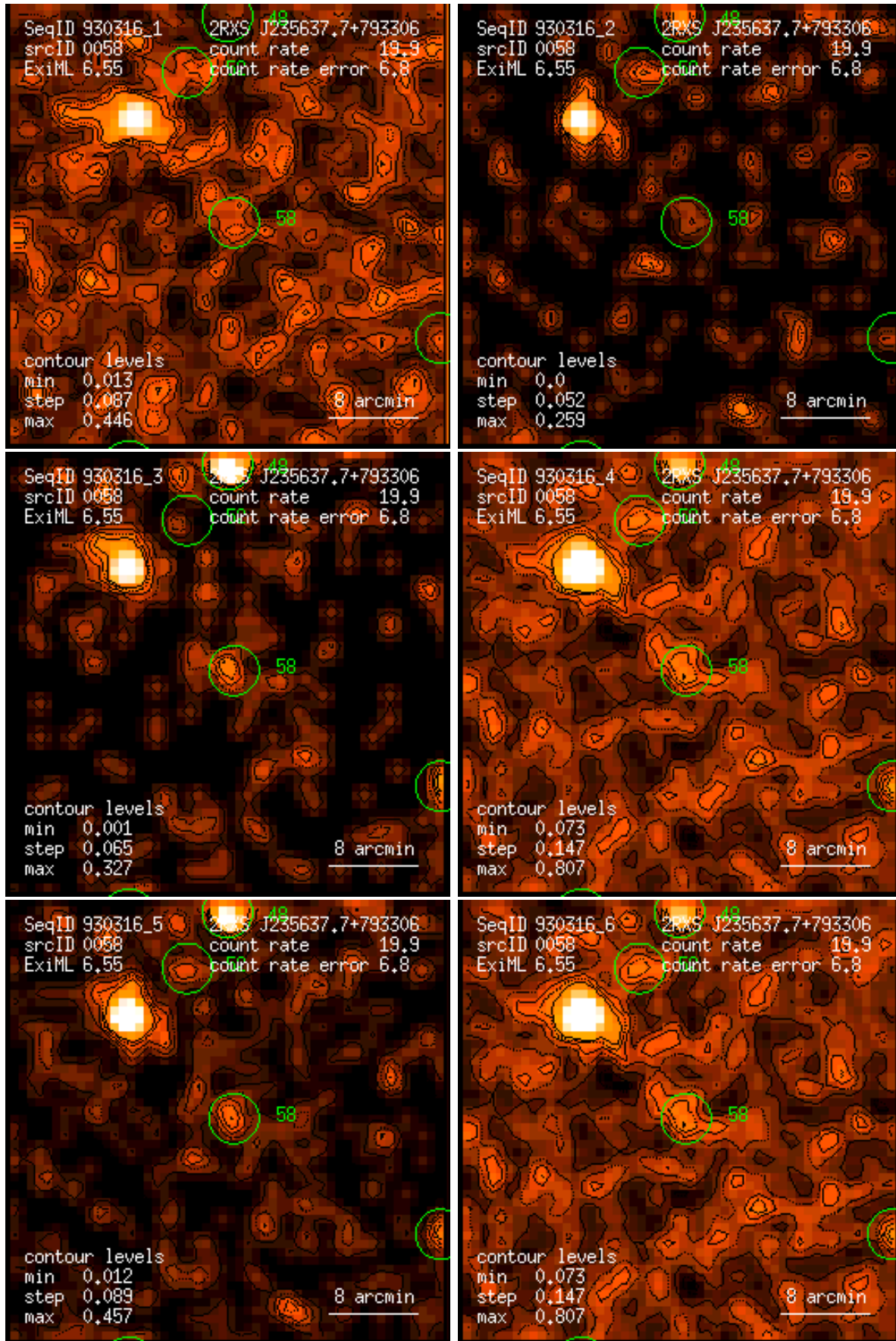
Figure 58: RASS 930316: detection 0058: band rate images, Gaussian filter: (1) PSPC channels 11 – 41, (2) 52 – 90, (3) 91 – 201, (4) 11 – 235, (5) 52 – 201, (6) 11 – 201. Broad band rates in counts/ks. Band rate contour levels in counts/ks/arcmin 2 .
