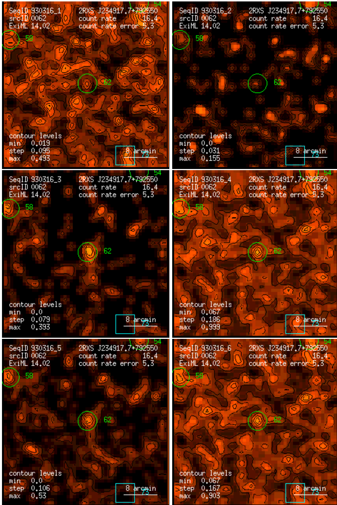
Figure 62: RASS 930316: detection 0062: band rate images, Gaussian filter: (1) PSPC channels 11 – 41, (2) 52 – 90, (3) 91 – 201, (4) 11 – 235, (5) 52 – 201, (6) 11 – 201. Broad band rates in counts/ks. Band rate contour levels in counts/ks/arcmin 2 .
