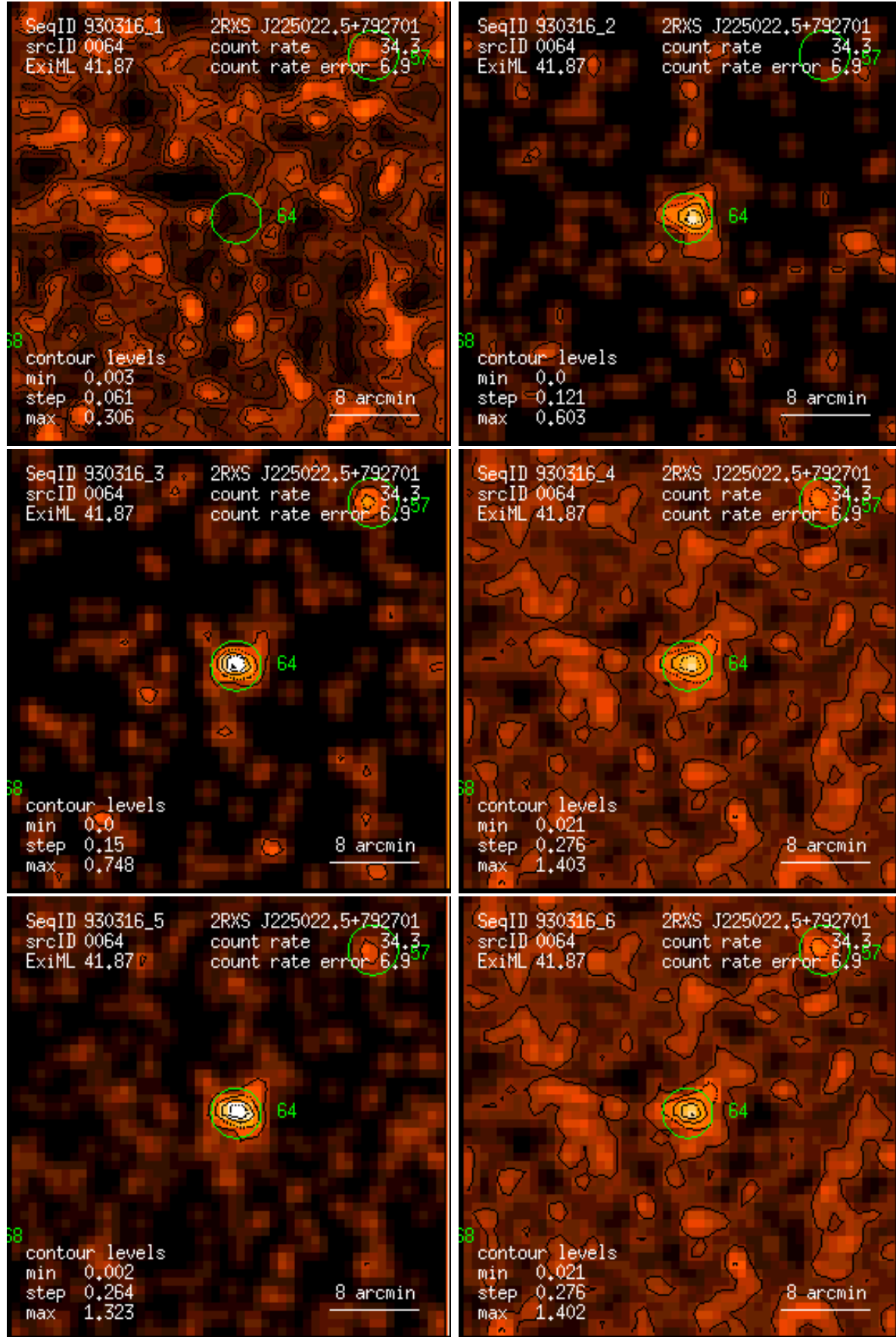
Figure 64: RASS 930316: detection 0064: band rate images, Gaussian filter: (1) PSPC channels 11 – 41, (2) 52 – 90, (3) 91 – 201, (4) 11 – 235, (5) 52 – 201, (6) 11 – 201. Broad band rates in counts/ks. Band rate contour levels in counts/ks/arcmin 2 .
