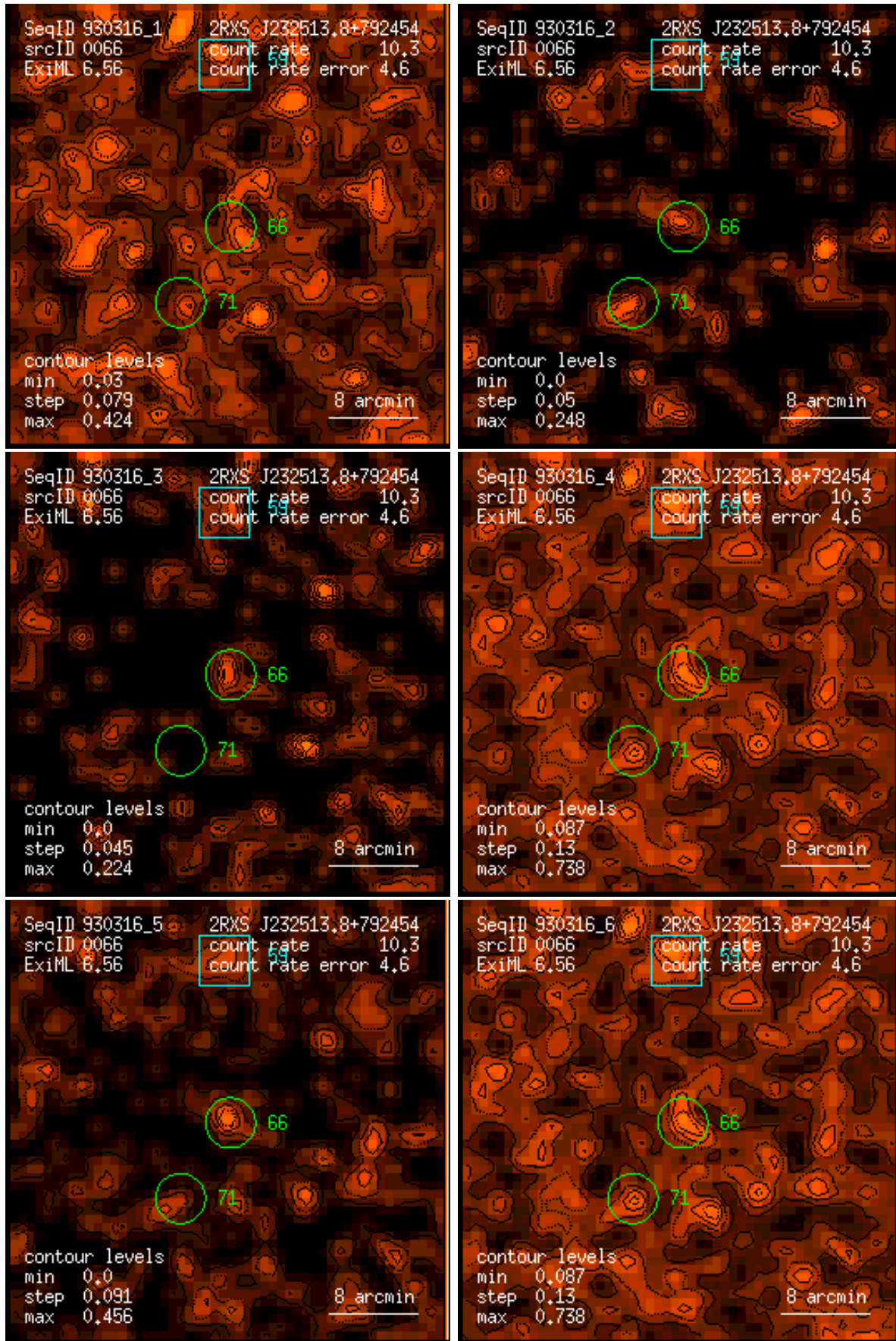
Figure 66: RASS 930316: detection 0066: band rate images, Gaussian filter: (1) PSPC channels 11 – 41, (2) 52 – 90, (3) 91 – 201, (4) 11 – 235, (5) 52 – 201, (6) 11 – 201. Broad band rates in counts/ks. Band rate contour levels in counts/ks/arcmin 2 .
