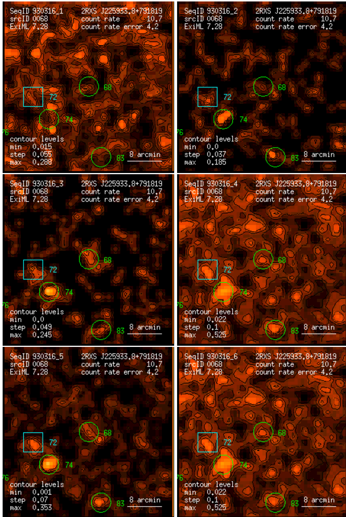
Figure 68: RASS 930316: detection 0068: band rate images, Gaussian filter: (1) PSPC channels 11 – 41, (2) 52 – 90, (3) 91 – 201, (4) 11 – 235, (5) 52 – 201, (6) 11 – 201. Broad band rates in counts/ks. Band rate contour levels in counts/ks/arcmin 2 .
