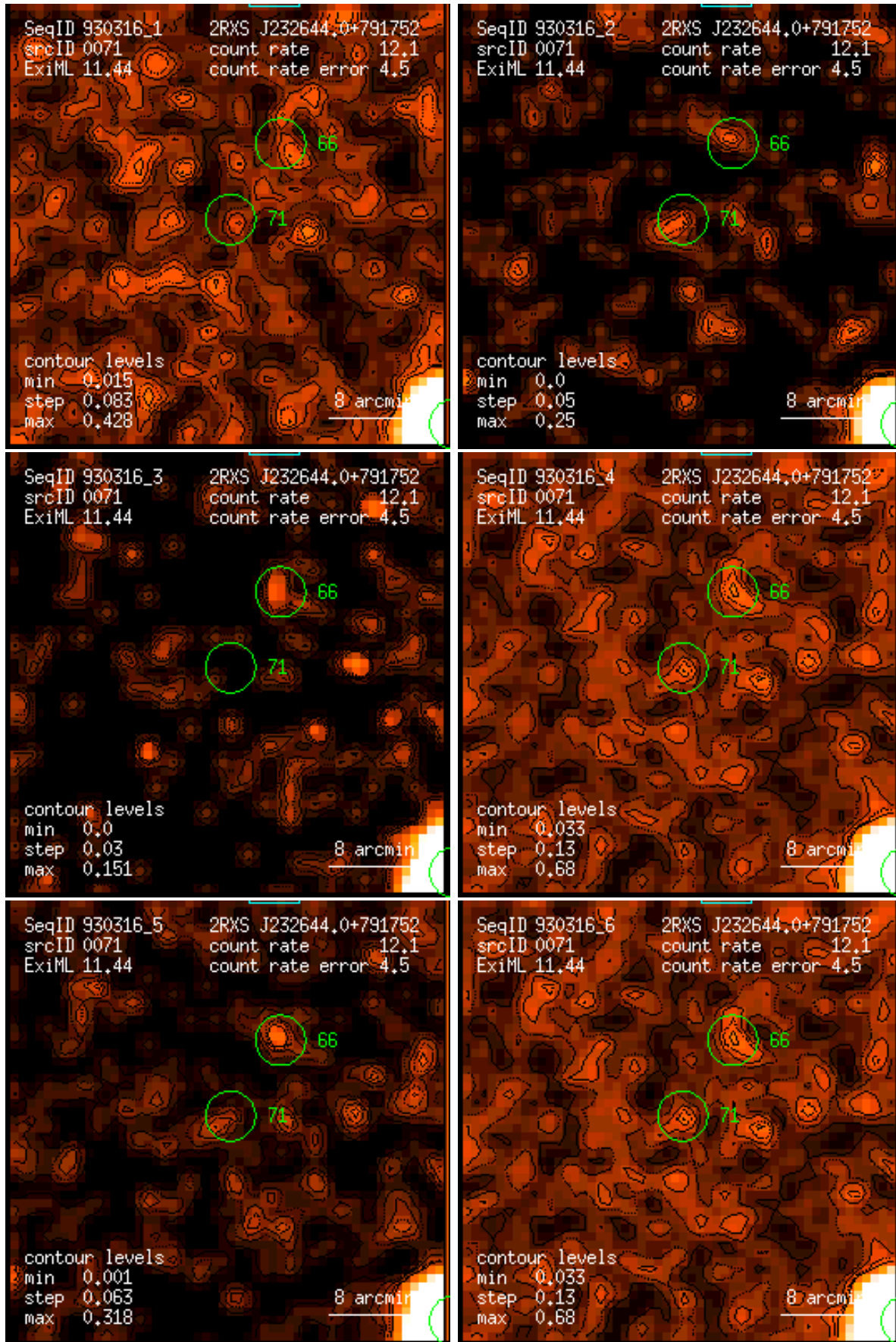
Figure 71: RASS 930316: detection 0071: band rate images, Gaussian filter: (1) PSPC channels 11 – 41, (2) 52 – 90, (3) 91 – 201, (4) 11 – 235, (5) 52 – 201, (6) 11 – 201. Broad band rates in counts/ks. Band rate contour levels in counts/ks/arcmin 2 .
