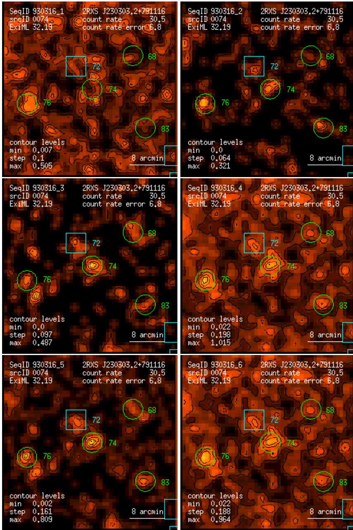
Figure 74: RASS 930316: detection 0074: band rate images, Gaussian filter: (1) PSPC channels 11 – 41, (2) 52 – 90, (3) 91 – 201, (4) 11 – 235, (5) 52 – 201, (6) 11 – 201. Broad band rates in counts/ks. Band rate contour levels in counts/ks/arcmin 2 .
