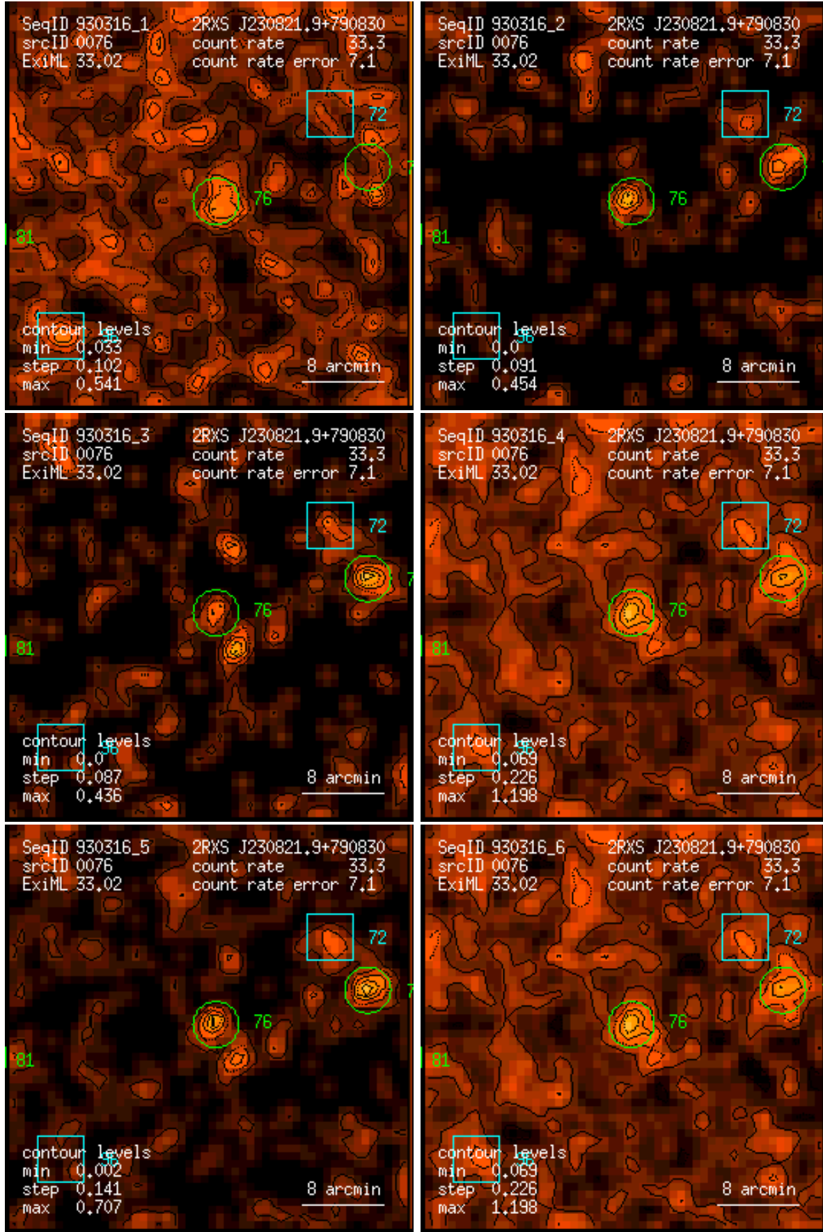
Figure 76: RASS 930316: detection 0076: band rate images, Gaussian filter: (1) PSPC channels 11 – 41, (2) 52 – 90, (3) 91 – 201, (4) 11 – 235, (5) 52 – 201, (6) 11 – 201. Broad band rates in counts/ks. Band rate contour levels in counts/ks/arcmin 2 .
