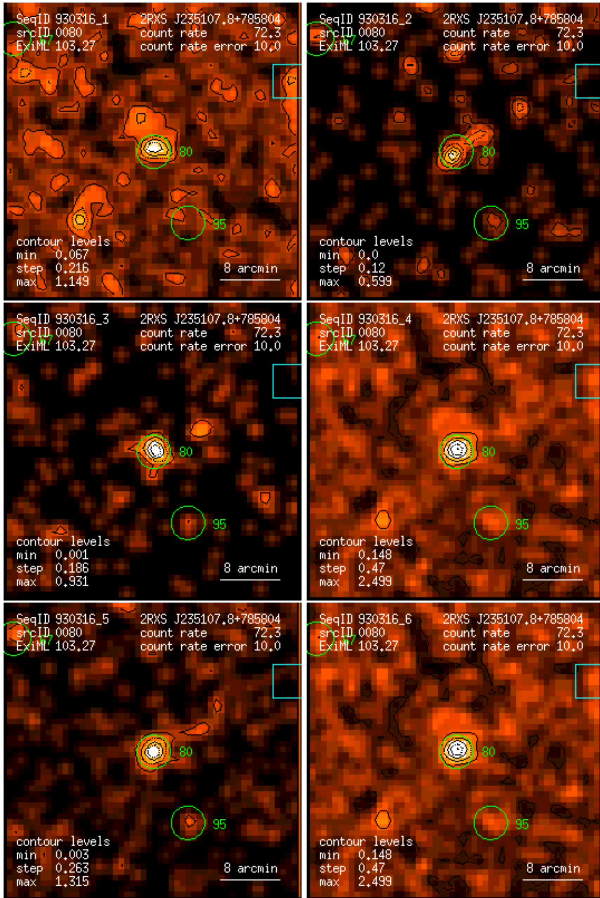
Figure 80: RASS 930316: detection 0080: band rate images, Gaussian filter: (1) PSPC channels 11 – 41, (2) 52 – 90, (3) 91 – 201, (4) 11 – 235, (5) 52 – 201, (6) 11 – 201. Broad band rates in counts/ks. Band rate contour levels in counts/ks/arcmin 2 .
