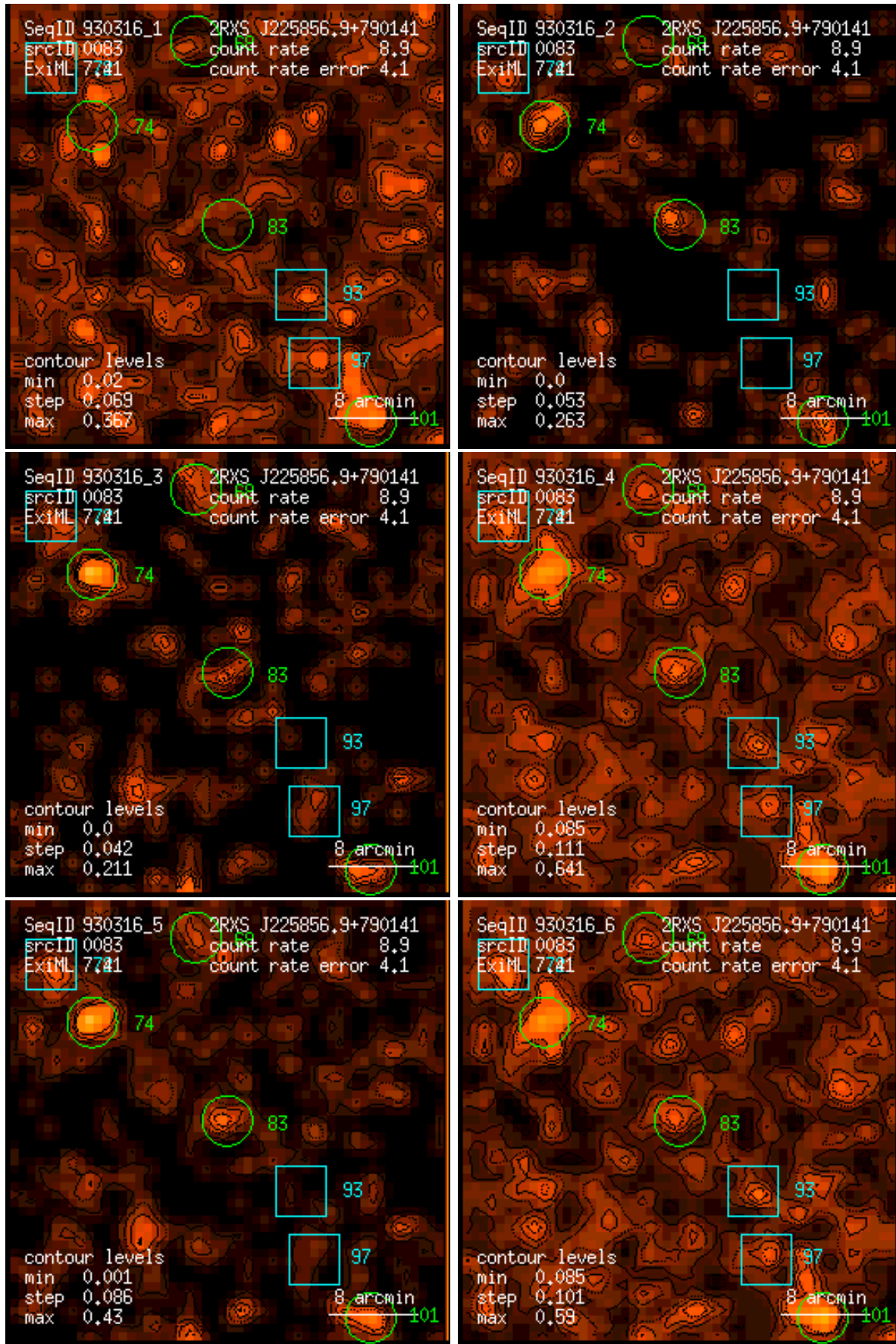
Figure 83: RASS 930316: detection 0083: band rate images, Gaussian filter: (1) PSPC channels 11 – 41, (2) 52 – 90, (3) 91 – 201, (4) 11 – 235, (5) 52 – 201, (6) 11 – 201. Broad band rates in counts/ks. Band rate contour levels in counts/ks/arcmin 2 .
