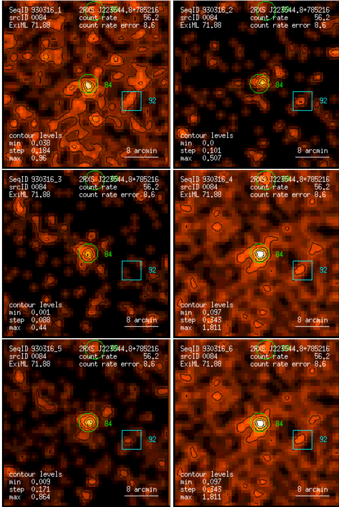
Figure 84: RASS 930316: detection 0084: band rate images, Gaussian filter: (1) PSPC channels 11 – 41, (2) 52 – 90, (3) 91 – 201, (4) 11 – 235, (5) 52 – 201, (6) 11 – 201. Broad band rates in counts/ks. Band rate contour levels in counts/ks/arcmin 2 .
