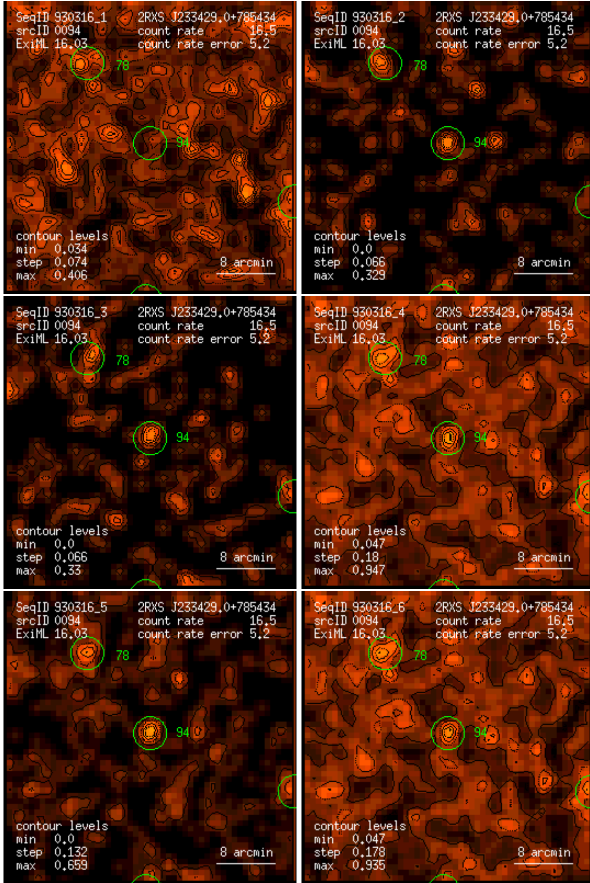
Figure 94: RASS 930316: detection 0094: band rate images, Gaussian filter: (1) PSPC channels 11 – 41, (2) 52 – 90, (3) 91 – 201, (4) 11 – 235, (5) 52 – 201, (6) 11 – 201. Broad band rates in counts/ks. Band rate contour levels in counts/ks/arcmin 2 .
