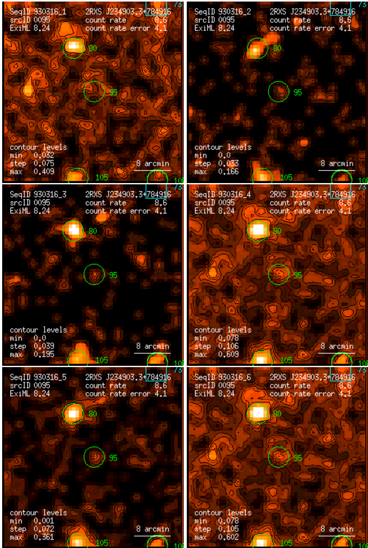
Figure 95: RASS 930316: detection 0095: band rate images, Gaussian filter: (1) PSPC channels 11 – 41, (2) 52 – 90, (3) 91 – 201, (4) 11 – 235, (5) 52 – 201, (6) 11 – 201. Broad band rates in counts/ks. Band rate contour levels in counts/ks/arcmin 2 .
