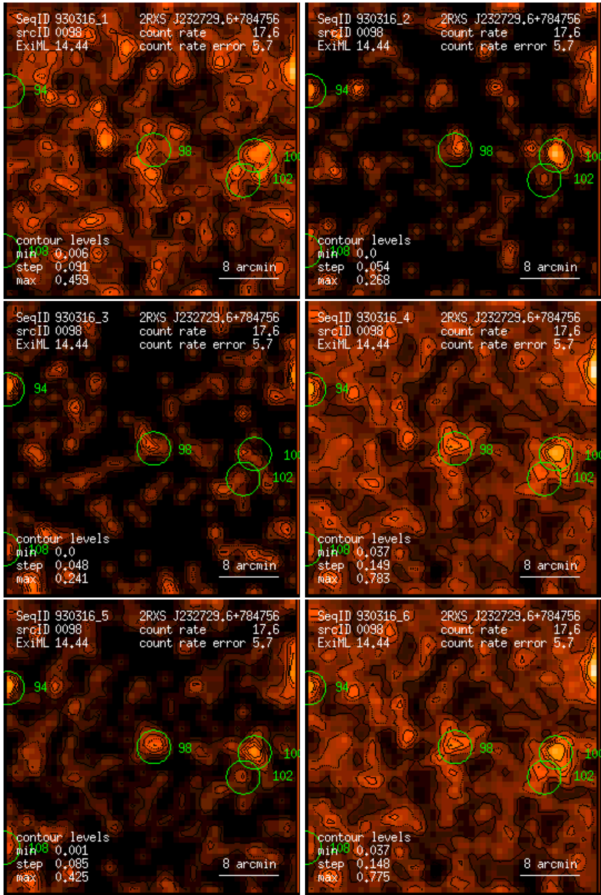
Figure 98: RASS 930316: detection 0098: band rate images, Gaussian filter: (1) PSPC channels 11 – 41, (2) 52 – 90, (3) 91 – 201, (4) 11 – 235, (5) 52 – 201, (6) 11 – 201. Broad band rates in counts/ks. Band rate contour levels in counts/ks/arcmin 2 .
