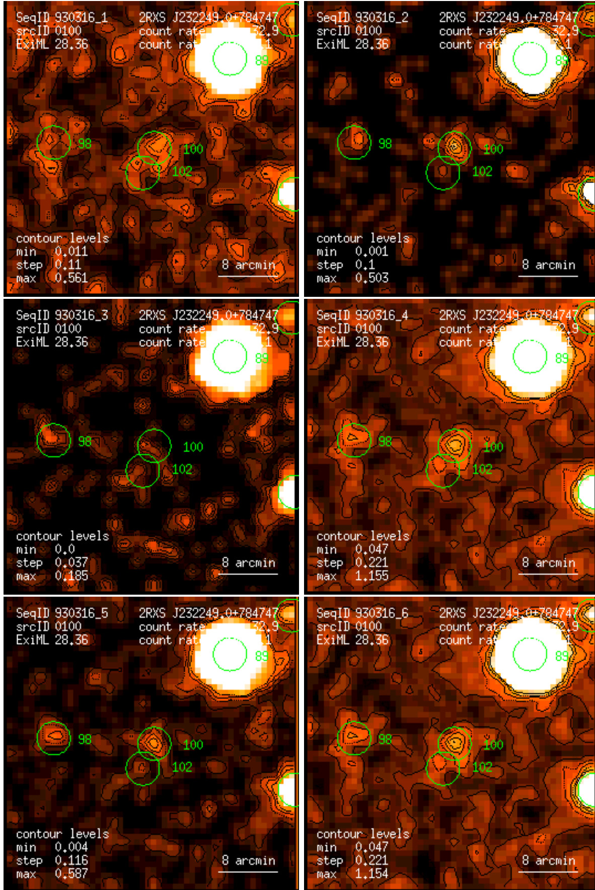
Figure 100: RASS 930316: detection 0100: band rate images, Gaussian filter: (1) PSPC channels 11 – 41, (2) 52 – 90, (3) 91 – 201, (4) 11 – 235, (5) 52 – 201, (6) 11 – 201. Broad band rates in counts/ks. Band rate contour levels in counts/ks/arcmin 2 .
